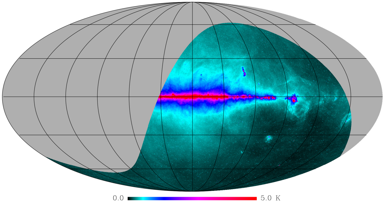
Figure 21. S-PASS Stokes I image. The map is in Mollweide projection, Galactic coordinates, with the Galactic centre at the centre and longitude increasing leftward.
