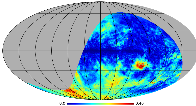
Figure 27. Fractional polarization L/I from S-PASS.
