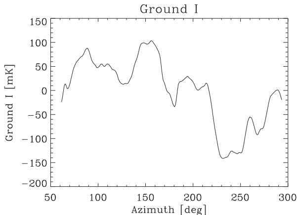
Figure 15. Ground-emission profile of Stokes I . Details are as for Fig. 13.
