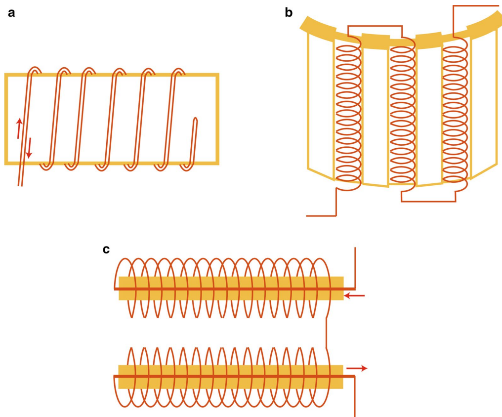
Fig. 1 Configuration of non-inductive heating wires. a Bifilar solenoid wrapped for a small oven, b solenoid-like helical heating wires arranged in a larger oven, c the new straight core solenoid heating wires using in the TD-PGL-100. Arrows indicate the current flow direction
