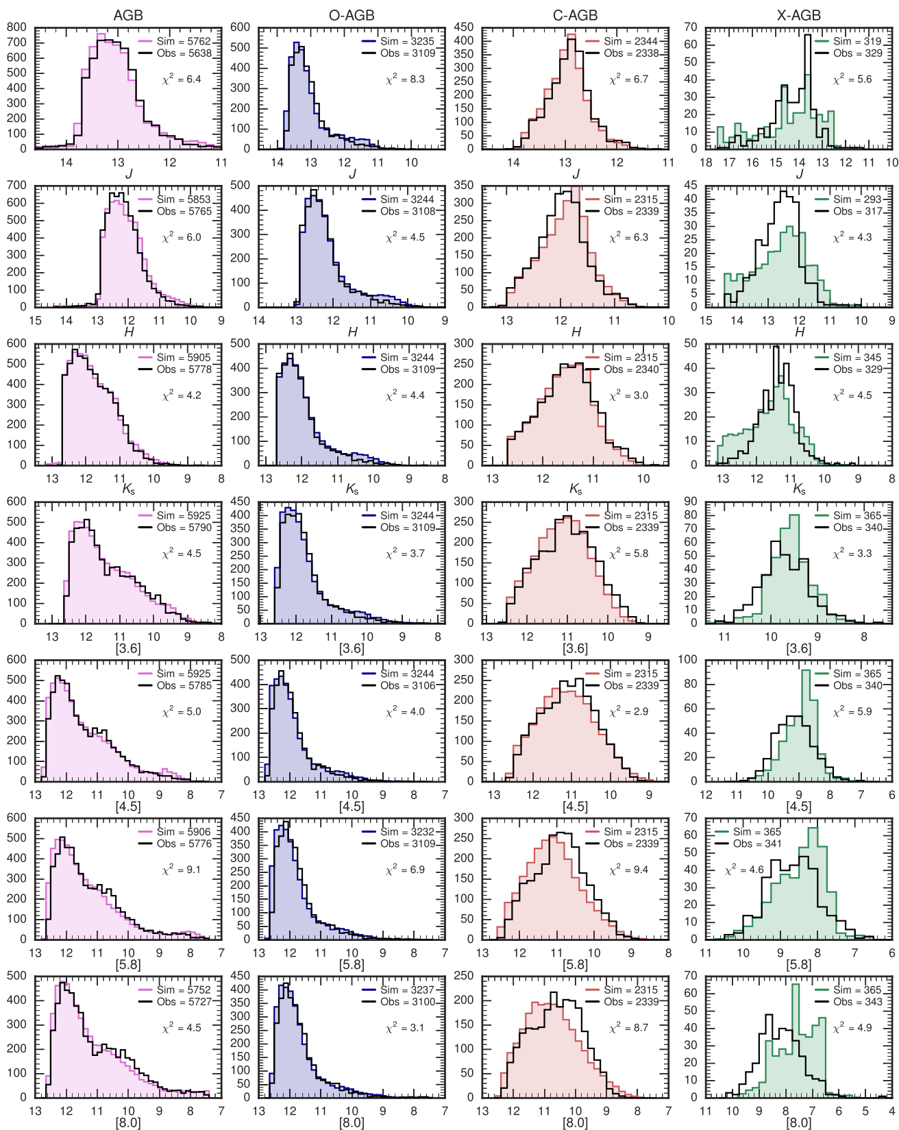
Figure 21. Comparison between the synthetic LFs obtained from the best-fitting model S 35 and the observed LFs in the 2MASS and Spitzer filters, going from shorter (top panels) to longer wavelengths (bottom panels).
