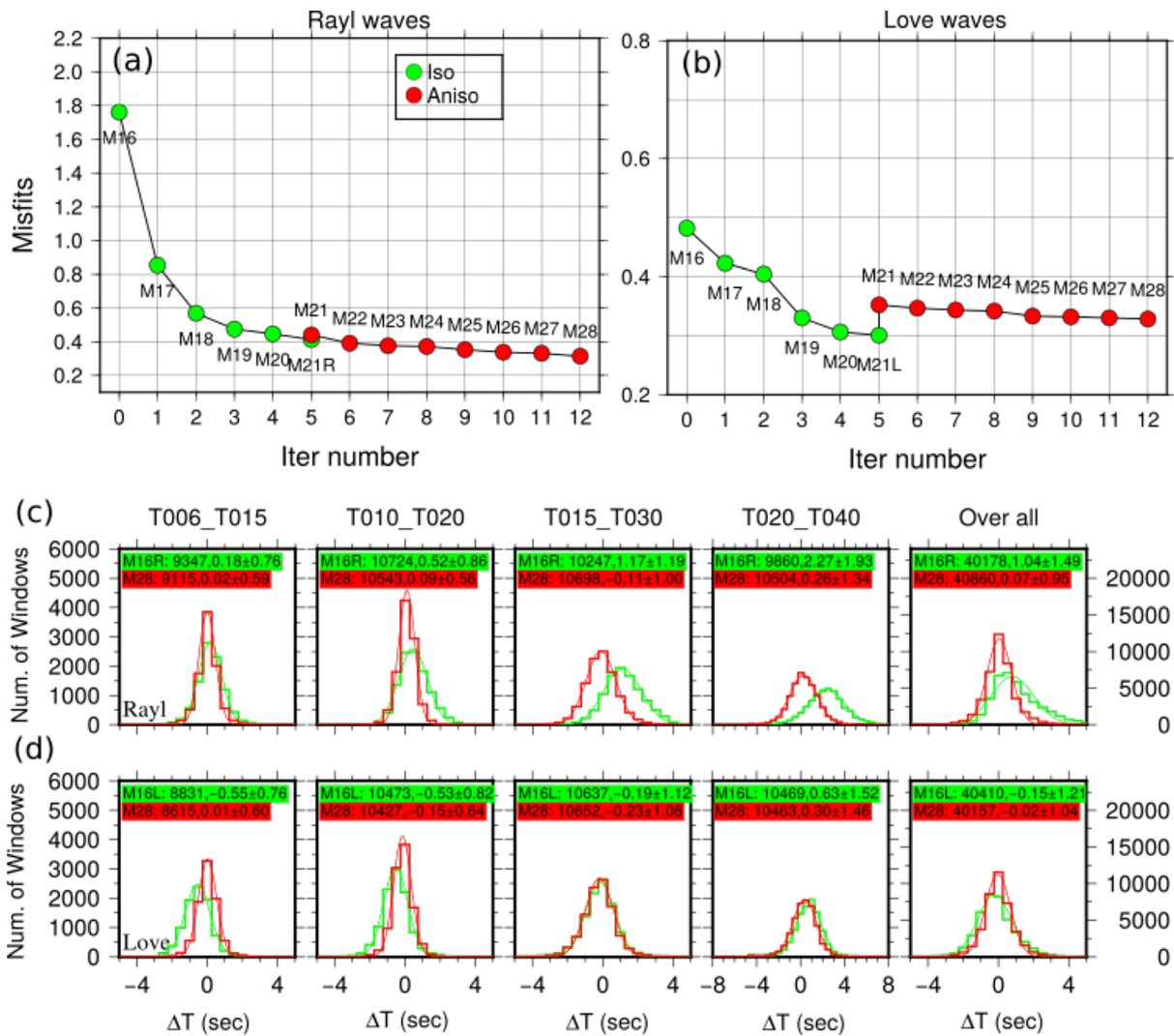
Figure 2. (a and b) The total traveltime misfit evolution over iterations for measurements between EGFs and SGFs made from Z-Z component Rayleigh waves and T-T component Love waves, respectively. The green solid circles are from isotropic inversions based on Rayleigh wave ANAT (Wang et al., 2018) and Love wave ANAT (Wang et al., 2019), and the red solid circles are from anisotropic inversion in this study. Note the total misfits of Rayleigh and Love waves increase a little for model M21 relative to the isotropic models ( M21R / M21L ) with more period bands data used and the introduction of radial anisotropy. (c and d) The differential traveltime histograms of different models for Rayleigh and Love waves, respectively. The green bars represent the traveltime histograms for the initial isotropic model M16 and the red bars are the corresponding traveltime histograms for our final anisotropic model M28 . The histograms are measured at four narrow period bands plotted in different columns, and the overall histograms are presented in the last column. The number of measurements, average value, and standard deviations are also shown in colored text boxes.
