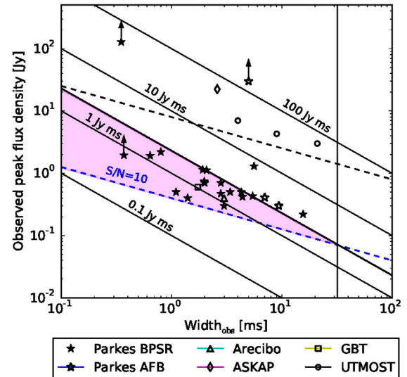
Figure 7. The observed peak flux density and observed width for all known FRBs. The sensitivity limits and fluence completeness region for BPSR Parkes events are indicated. These do not apply to other events which are shown for reference only.
