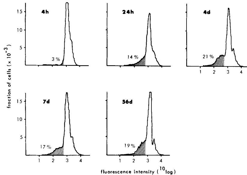
FIG. 4. Neonatal thymus rapidly acquires a dull \text{Thy-1}^+ population similar in size to the dull \text{Thy-1}^+ population in adults. (For analysis details, see legend to Fig. 3.)
