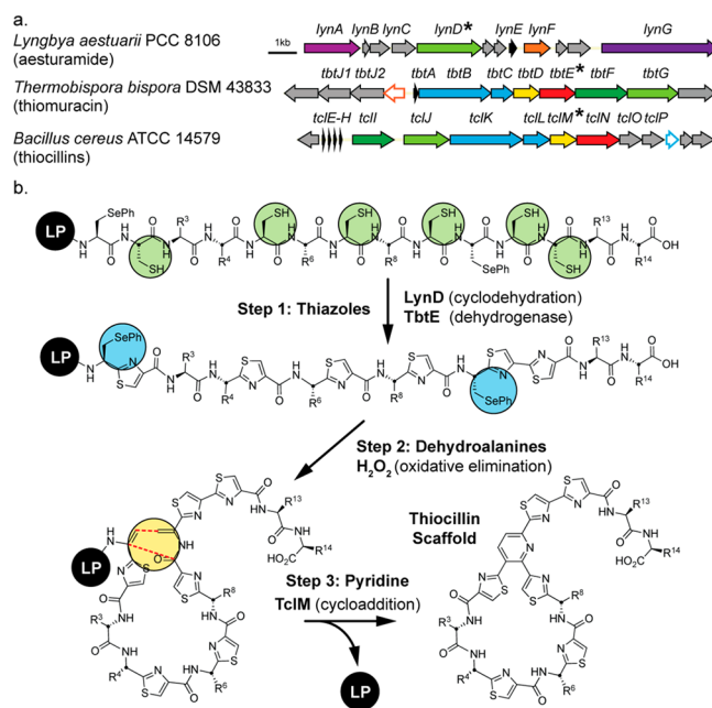
Figure 1. Flexizyme-enabled benchtop biosynthesis of thiopeptide scaffolds. (a) Biosynthetic gene clusters of thiocillins, thiomuracin GZ, and aesturamide. Genes for key enzymes used in this work are highlighted with asterisks. (b) Proposed hybrid route to the thiocillin core.
