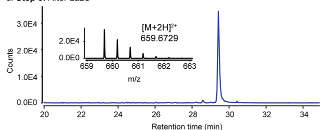
Figure 3. Flexizyme-enabled benchtop biosynthesis of lactazole W2S, S11C. (a) Sequence of designer precursor peptide. (b) Proposed route to lactazole scaffolds. EICs for the hexathiazole and Dha-containing product of treatment with LynD/TbtE and H 2 O 2 (c) and fully cyclized lactazole core (d).
