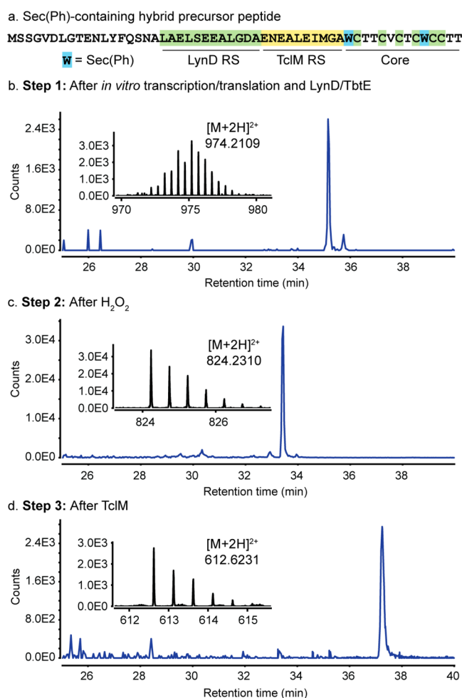
Figure 2. Flexizyme-enabled benchtop biosynthesis of a thiocillin scaffold. (a) Sequence of the designer precursor peptide, including a pMCSG7-derived sequence, the LynD RS, and TcIM RS. The Trp-codon was reprogrammed to incorporate SecPh. EICs for SecPh and hexathiazole precursor peptide after LynD/TbtE treatment (b), hexathiazole and Dha-containing product after oxidative elimination (c), and fully cyclized thiocillin core (d).
