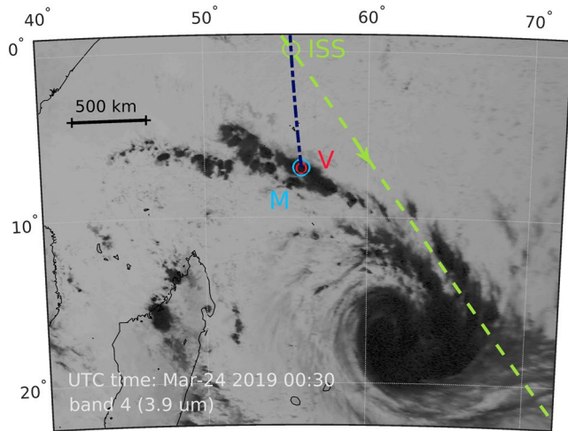
Figure 1. Image from geostationary satellite Meteosat-11 around 00:30 UTC, about 1 min and 53 s before the ASIM trigger. The image comes from the optical band 4 (3.9 \mu\text{m} , 3 km resolution). The tropical cyclone Joaninha can be seen in the south-east part of the picture and extends over a thousand of kilometers. The positions of the ISS, the GLD360 match (V), and the magnetic field line footpoint (M) are indicated. The track of the Earth's magnetic field line (dark blue dashed line) and of the trajectory of the ISS (green dashed line) are also showed. Point V is very close to M in both location ( \Delta r = 4.82 km) and time ( \Delta t = 1.44 m s), and is located in the north-western rainbands of the cyclone. ISS, International Space Station.
