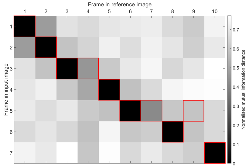
Fig. 4. Showing the values of the distance matrix which are used in the heuristic calculation for an example distance matrix. Darker squares represent a lower normalised mutual information distance and a better match between frames. Note how the resulting "path" would be invalid, as it is not monotonic, but meets the condition of being a lower limit to the optimal cost.
