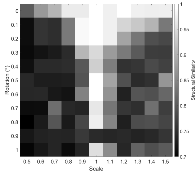
Fig. 13. Showing how differences in rotation and scale between the reference image and image strips can reduce the quality of the correction. Lighter squares represent better results and darker squares show a worse result.
