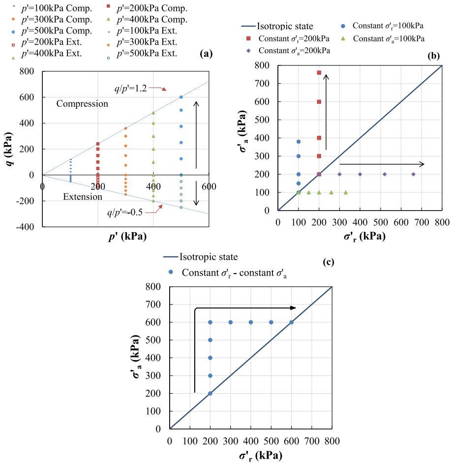
Fig. 5. Illustration of the anisotropic stress paths followed (the data points represent the stress states where binder element tests were conducted): (a) Constant p' compression and extension stress paths on the q - p' plane, (b) Constant \sigma'_a and constant \sigma'_r stress paths on the \sigma'_a - \sigma'_r plane, and (c) Constant \sigma'_r -constant \sigma'_a stress path on the \sigma'_a - \sigma'_r plane.
