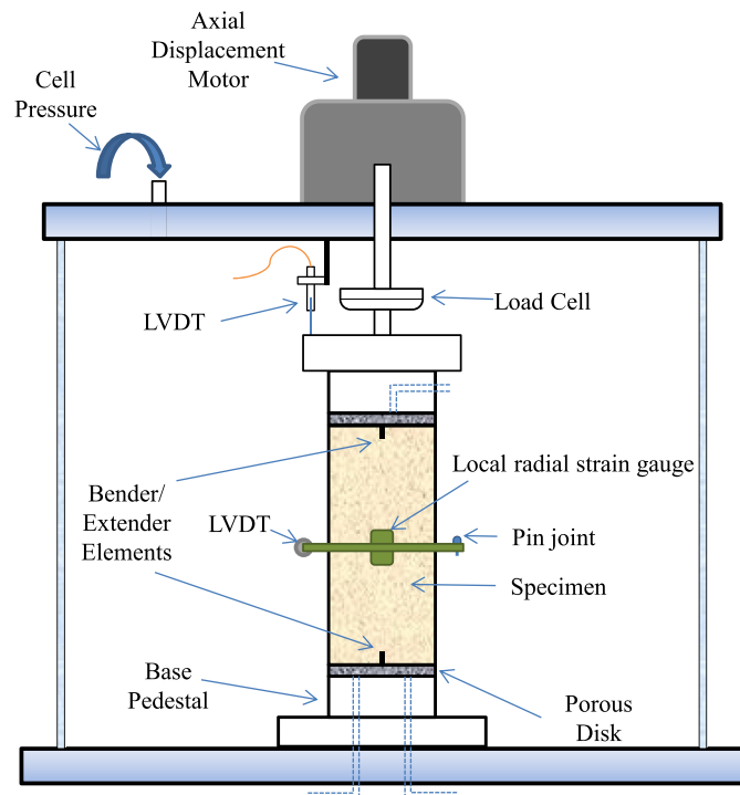
Fig. 2. Schematic illustration of the dynamic triaxial system with the local strain gauge (specimen diameter: 50 mm; specimen height: 100 mm).
