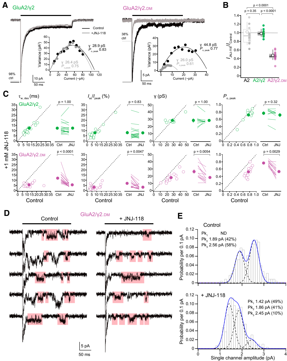
Fig. 6. A double point mutation in TARP \gamma 2 introduces JNJ-118 sensitivity to GluA2(Q)/ \gamma 2 . (A) Representative outside-out patch responses (10 mM glutamate, 200 milliseconds) (black bars) recorded at -60 mV from HEK293 cells transfected with GluA2/ \gamma 2 (left) or GluA2/ \gamma 2 .DM (right) in control conditions (black) or in the presence of 1 \mu\text{M} JNJ-118 (gray). Insets show corresponding current-variance relationships and estimated channel conductance ( \gamma ) and peak open probability ( P_{o, peak} ). (B) Pooled peak inhibition data ( I_{JNJ-118}/I_{Control} ) showing the effect of 1 \mu\text{M} JNJ-118 on GluA2 alone (from Fig. 1B), GluA2/ \gamma 2 , and GluA2/ \gamma 2 .DM. Box-and-whisker plots as in Fig. 1. Indicated P values are from two-sided Wilcoxon rank-sum tests (adjusted for multiple comparisons as described in Table 1) following a nonparametric omnibus test (Supplemental Table 1). (C) Scatter and paired plots (as in Fig. 2) showing the effects of 1 \mu\text{M} JNJ-118 on the weighted mean time constant of desensitization ( \tau_{w, des} ), the fractional steady-state component ( I_{ss}/I_{peak} ), the weighted mean channel conductance, and P_{o, peak} values for GluA2/ \gamma 2 and GluA2/ \gamma 2 .DM. Indicated P values are from two-sided Wilcoxon signed-rank exact tests (adjusted as described in Table 1) following a nonparametric omnibus test (Supplemental Table 1). (D) Representative responses (10 mM glutamate, 200 milliseconds; black bars) recorded at -60 mV from an outside-out patch expressing GluA2/ \gamma 2 .DM in the presence and absence of 1 \mu\text{M} JNJ-118. Five consecutive sweeps are shown in each condition; the initial peak is truncated, and selected single-channel openings are highlighted. Note the prevalence of lower amplitude events in the presence of JNJ-118. (e) Pooled amplitude histograms of resolved GluA2/ \gamma 2 .DM openings in the absence (top) and presence (bottom) of JNJ-118 (228 and 289 openings from 2 and 3 patches, respectively). Note the skew in amplitudes toward lower values in the presence of JNJ-118. Dotted black lines are individual gaussian fits with indicated means and proportions. Solid blue lines are the sums of the fitted gaussians.
