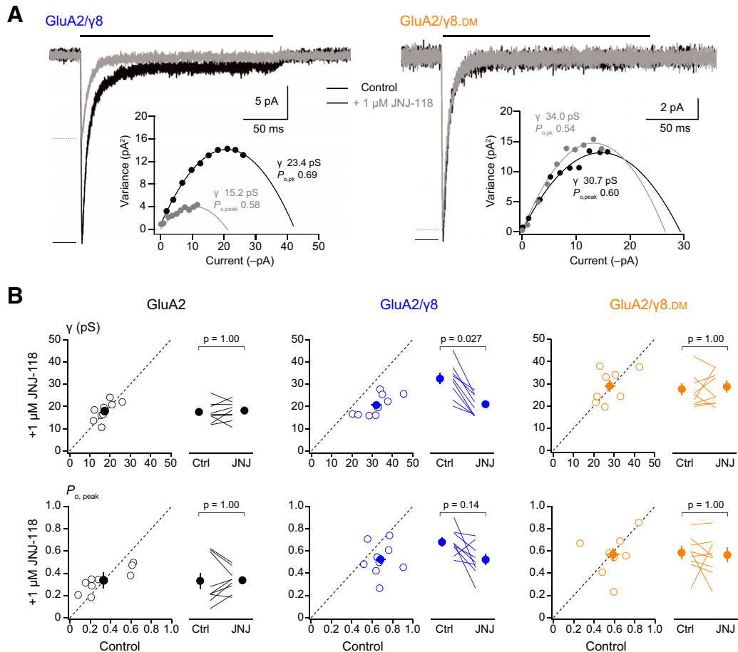
Fig. 2. JNJ-118 decreases the weighted mean channel conductance of GluA2(Q)/ \gamma 8. (A) Representative outside-out patch responses (10 mM glutamate, 200 milliseconds) (black bars) recorded at -60 mV from HEK293 cells transfected with GluA2/ \gamma 8 (left) or GluA2/ \gamma 8.DM (right) in control conditions (black) or in the presence of 1 \mu\text{M} JNJ-118 (gray). Insets show corresponding current-variance relationships and estimated channel conductance ( \gamma ) and peak open probability ( P_{o,\text{peak}} ). (B) Scatter and paired plots showing the effects of 1 \mu\text{M} JNJ-118 on weighted mean channel conductance ( \gamma ) and P_{o,\text{peak}} values for GluA2, GluA2/ \gamma 8, and GluA2/ \gamma 8.DM. Open circles show individual values, and filled circles denote the means, with error bars indicating S.E.M. In scatter plots, dashed lines denote equality, with points below the lines indicating inhibitory effects of JNJ-118. Indicated P values (adjusted for multiple comparisons as described in Table 1) are from two-sided Wilcoxon signed-rank exact tests following a nonparametric omnibus test (Supplemental Table 1).
