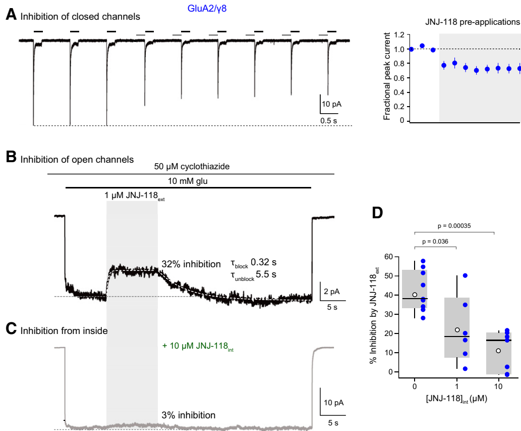
Fig. 5. Inhibition by JNJ-118 is unaffected by channel state, and the drug is effective when applied intracellularly. (A) Representative concatenated responses from a GluA2/ \gamma 8 outside-out patch evoked by applications of 10 mM glutamate (200 milliseconds, 1 Hz; black bars) at -60 mV, showing inhibition produced by preapplications of 1 \mu M JNJ-118 (200 milliseconds; gray bars). Right-hand panel shows mean peak current data from 7 records (error bars indicate S.E.M.), normalized in each case to the mean of three applications delivered before the first preapplication of JNJ-118. (B) Representative response from a GluA2/ \gamma 8 outside-out patch produced by a 48-second application of 10 mM glutamate (black bar) in the constant presence of 50 \mu M cyclothiazide. Filled gray area denotes the rapid application of 1 \mu M JNJ-118 for 10 seconds. White dotted lines are single exponential fits showing the timecourse of block and unblock. (C) Representative response, as in panel B, but recorded with an internal solution containing 10 \mu M JNJ-118. Note that in this case, the extracellular application of JNJ-118 produced a greatly reduced block. (D) Pooled data showing the degree of inhibition produced by 1 \mu M JNJ-118 ext when the internal solution contained either 0, 1, or 10 \mu M JNJ-118. Box-and-whisker plots as in Fig. 1. Indicated P values (adjusted for multiple comparisons using Holm's sequential Bonferroni correction) are from two-sided Wilcoxon rank-sum tests following Kruskal-Wallis rank-sum test (Supplemental Table 1).
