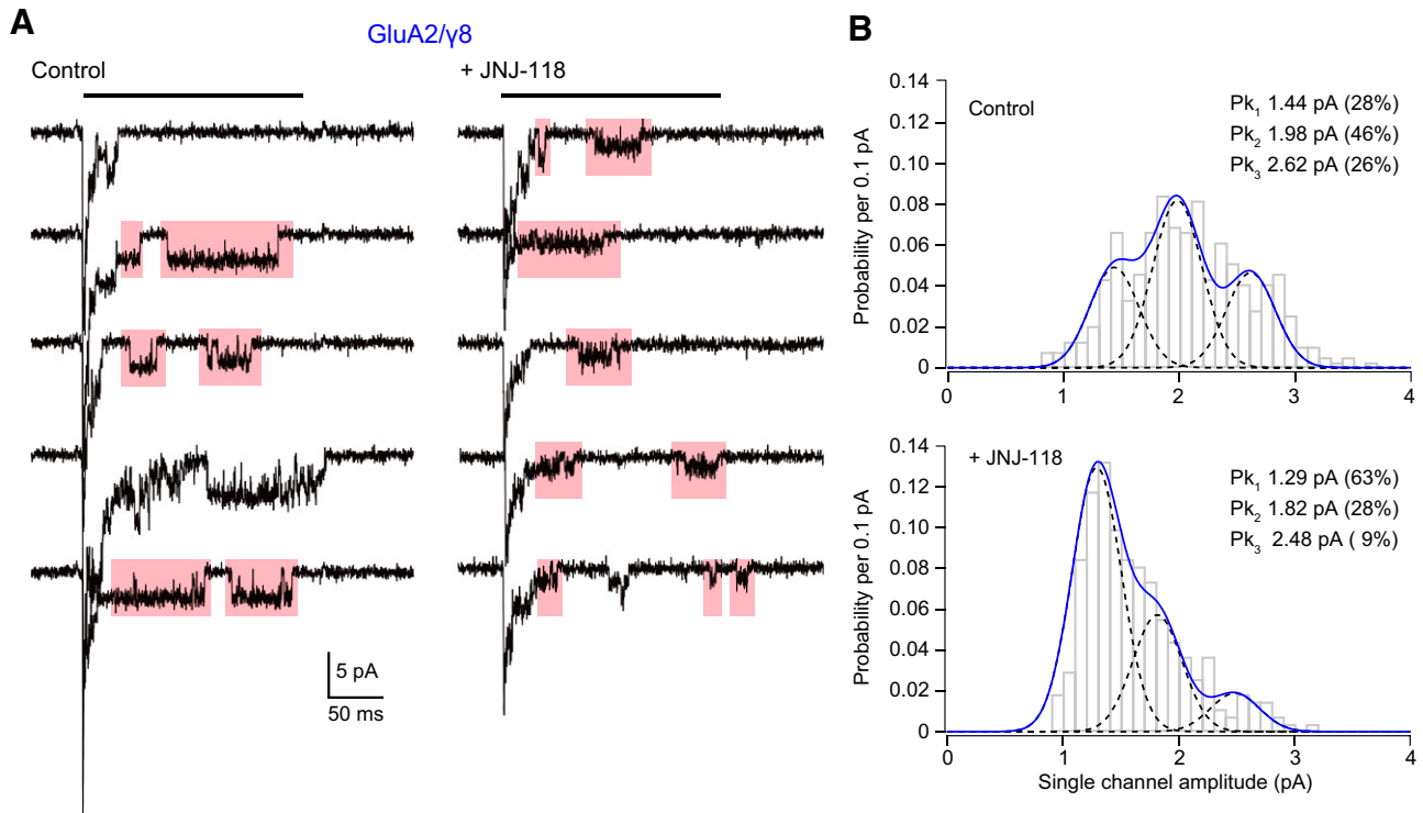
Fig. 3. JNJ-118 reduces the prevalence of higher conductance openings of GluA2(Q)/ \gamma 8 channels. (A) Representative responses (10 mM glutamate, 200 milliseconds; black bars) recorded at -60 mV from an outside-out patch expressing GluA2/ \gamma 8 in the presence and absence of 1 \mu\text{M} JNJ-118. Five consecutive sweeps are shown in each condition; the initial peak is truncated, and the single-channel openings from these sweeps that were included in the analysis are highlighted. Note the prevalence of lower amplitude events in the presence of JNJ-118. (B) Pooled amplitude histograms of resolved GluA2/ \gamma 8 openings in the absence (top) and presence (bottom) of JNJ-118 (392 and 272 openings from 8 and 6 patches, respectively). Note the skew in amplitudes toward lower values in the presence of JNJ-118. Dotted black lines are individual gaussian fits with indicated means and proportions. Solid blue lines are the sums of the fitted gaussians.
