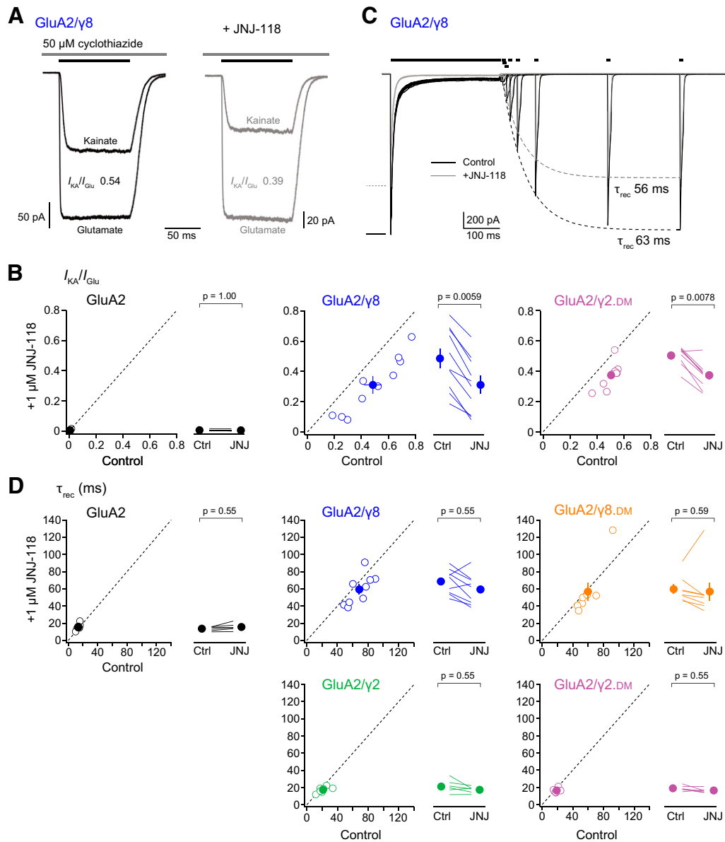
Fig. 7. JNJ-118 influences kainate relative efficacy but not recovery from desensitization. (A) Glutamate- and kainate-evoked currents ( -60 mV) recorded from the same representative patch in the presence of 50 \mu\text{M} cyclothiazide in the absence (left) and presence (right) of 1 \mu\text{M} JNJ-118. The glutamate responses are scaled to highlight the small decrease in the relative efficacy of kainate. (B) Scatter and paired plots (as in Fig. 2) showing the effects of 1 \mu\text{M} JNJ-118 on I_{KA}/I_{Glu} for GluA2, GluA2/ \gamma 8, and GluA2/ \gamma 2.DM. Indicated P values are from two-sided Wilcoxon signed-rank exact tests (adjusted for multiple comparisons as described in Table 1) following a nonparametric omnibus test (Supplemental Table 1). (C) Glutamate-evoked currents ( -60 mV) from a representative GluA2/ \gamma 8 outside-out patch demonstrating the time course of recovery following desensitization with 10 mM glutamate ( 250 milliseconds; black bar) in the absence and presence of 1 \mu\text{M} JNJ-118. Recovery of peak currents was assessed using glutamate reapplication ( 10 milliseconds; short black bars) at intervals from 2 – 500 milliseconds, and single exponentials (dashed lines) were fitted to the peak currents. (D) Scatter and paired plots showing the effects of 1 \mu\text{M} JNJ-118 on \tau_{rec} for GluA2, GluA2/ \gamma 8, GluA2/ \gamma 8.DM, GluA2/ \gamma 2 and GluA2/ \gamma 2.DM. Open circles show individual values, and filled circles denote the means, with error bars indicating S.E.M. In scatter plots, dashed lines denote equality, with points below the lines indicating inhibitory effects of JNJ-118. Indicated P values are from two-sided Wilcoxon signed-rank exact tests (adjusted as described in Table 1) following a nonparametric omnibus test (Supplemental Table 1).
