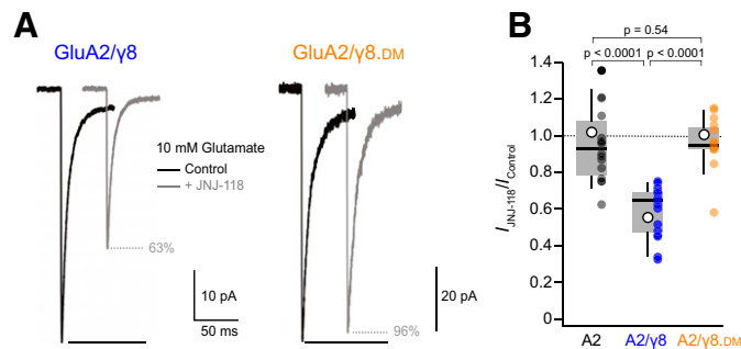
Fig. 1. JNJ-118 decreases peak amplitude of currents from GluA2(Q)/ \gamma 8 . (A) Representative outside-out patch responses (10 mM glutamate, 200 milliseconds, -60 mV) from two HEK293 cells transfected with GluA2/ \gamma 8 (left) or GluA2/ \gamma 8_{DM} (right) in control conditions (black) and in the presence of 1 \mu M JNJ-118 in both control and glutamate solutions (gray). Only the initial part of each response is shown, with the percent peak current remaining in JNJ-118 indicated. (B) Pooled peak inhibition data ( I_{JNJ-118}/I_{Control} ) showing the effect of 1 \mu M JNJ-118 on GluA2 alone, GluA2/ \gamma 8 , and GluA2/ \gamma 8_{DM} . Box-and-whisker plots indicate the median (black line), the 25th–75th percentiles (box), and the 10th–90th percentiles (whiskers); filled circles are data from individual patches, and open circles indicate means. Indicated P values (adjusted for multiple comparisons as described in Table 1) are from two-sided Wilcoxon rank-sum tests following a nonparametric omnibus test (Supplemental Table 1).
