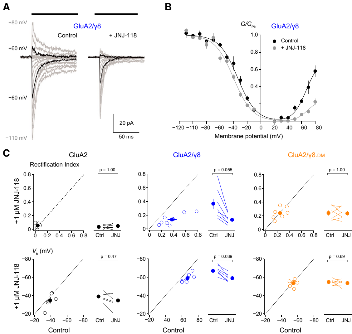
Fig. 4. JNJ-118 increases spermine block of GluA2(Q)/ \gamma 8 receptors. (A) Representative responses evoked by 10 mM glutamate (200 milliseconds; black bars) recorded at potentials between -110 mV and +80 mV from an outside-out patch in the absence (left) and presence (right) of 1 \mu\text{M} JNJ-118. In each case, the responses at -60 and +60 mV (from which RI was calculated) are shown in black. (B) Pooled normalized conductance-voltage relationships for GluA2/ \gamma 8 in the absence and presence of 1 \mu\text{M} JNJ-118. The filled symbols are the mean values from 6 cells (with error bars showing S.E.M.), and the solid lines are fits of double Boltzmann relationships (see Methods ). (C) Scatter and paired plots (as in Fig. 2) showing the effects of 1 \mu\text{M} JNJ-118 on Rectification Index and V_b (from individual double Boltzmann fitted conductance-voltage relationships) for GluA2, GluA2/ \gamma 8, and GluA2/ \gamma 8.DM. The indicated P values (adjusted for multiple comparisons as described in Table 1) are from two-sided Wilcoxon signed-rank exact tests following a nonparametric omnibus test (Supplemental Table 1).
