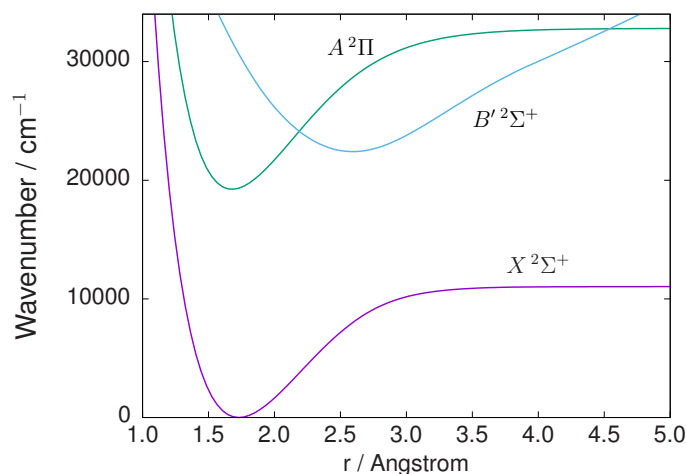
Figure 3. The empirically refined (adiabatic) potential energy curves of MgH. Note that the B'{}^2\Sigma^+ state displays incorrect dissociation behaviour (see text).
