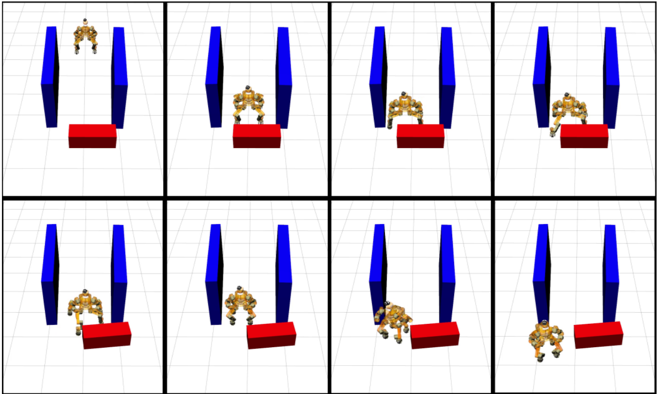
FIGURE 19. Simulation sequence depicting the robot moving through a corridor, clearing the obstructing object and moving forward. The robot first reaches the obstructing movable obstacle. It then expands and moves to the side to allow the front right wheel to use its full range of horizontal motion inwards to perform the push and then push the object from the side.
