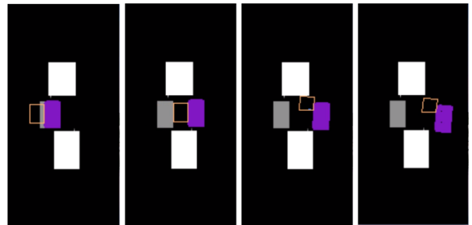
FIGURE 16. Image simulation sequence depicting a double legged drive through push sequence execution followed by a single legged rotating push to clear the robot of the initial planned path so as to allow the robot enough space to rejoin the planned again by going around the object.
