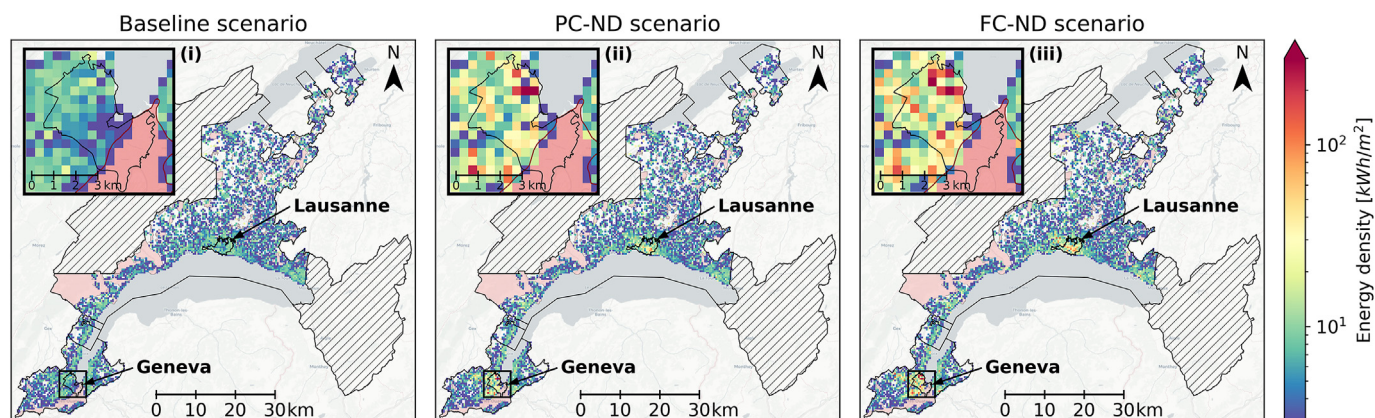
Fig. 5. Heat extraction potential ( Q_{opt} ) of individual GSHPs, aggregated to pixels of (400 \times 400) m 2 , for (a) baseline scenario (NC-ND), (b) partial cooling (PC-ND-4.5) and (c) full cooling scenario (FC-ND-4.5) in western Switzerland. In pink zones, GSHPs installation is prohibited.
