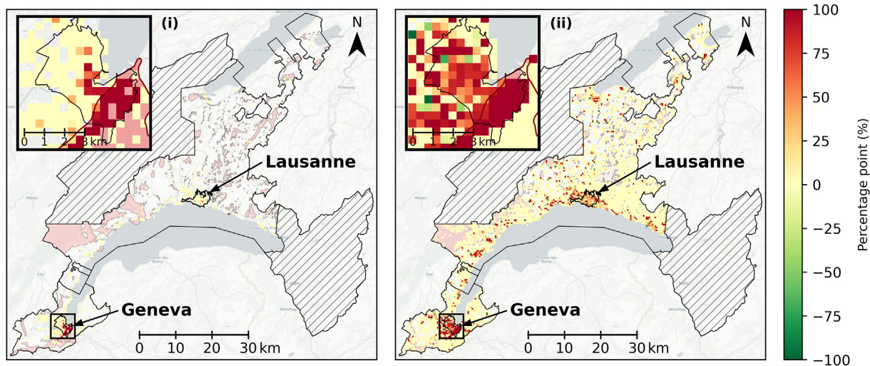
Fig. 11. The difference between PC-ND-4.5 and PC-D-4.5 scenarios: a) percentage of cooling demand supplied; b) percentage of heat demand supplied.
