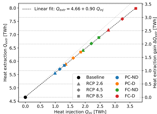
Fig. 7. Geothermal potential ( Q_{extr} ) as a function of injected excess heat ( Q_{inj} ), for all scenarios (see Table 2). The black dashed line shows the linear fit, the grey dashed line represents a slope of 1.
