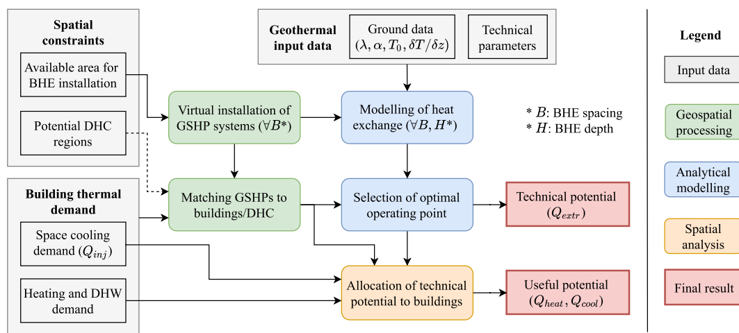
Fig. 1. Workflow for modelling the technical potential of GSHP ( Q_{extr} ) and the useful potential for supplying heat ( Q_{heat} ) and cooling ( Q_{cool} ), consisting of three stages: (1) Geospatial processing (green boxes), (2) Analytical modelling (blue boxes), and (3) Spatial analysis (orange box), corresponding to the following sub-sections. Dashed lines are used only if DHC is considered.
