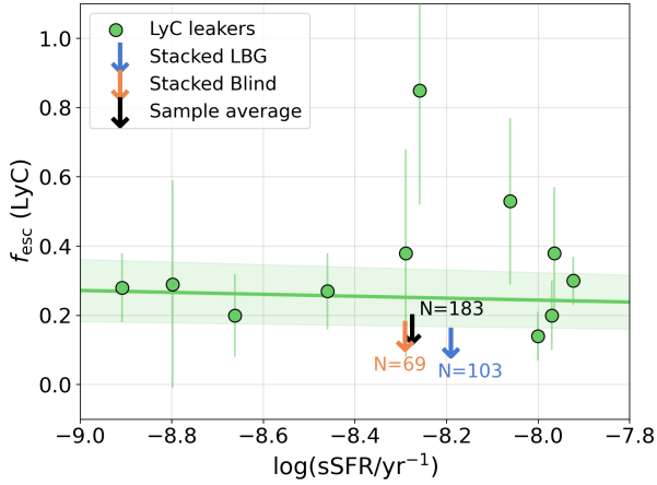
Figure 10. Distribution of f_{\text{esc}} and sSFR of candidate LyC leakers, LBG and blind-selected galaxies as well as the sample average (same legend as Figure 9). We find little to no correlation between f_{\text{esc}} and sSFR of individual LyC leakers at the 2\sigma confidence level, with a best-fit slope -0.028 \pm 0.015 (solid green line with uncertainty in shaded region). The stacked f_{\text{esc}} values derived from LBG and blind-selected samples are consistent with the best-fit relation. The lack of dependence of f_{\text{esc}} on sSFR has also been seen in simulations (e.g. Yoo et al. 2020).
