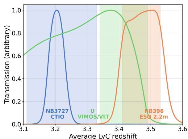
Figure 1. Filter transmission profiles of the NB3727 , NB396 and the U band filters used to target LyC emission in this study. The x-axis shows the redshift at the rest-frame wavelength of 886 Å, which is the mid-point wavelength of the LyC emission sampled between 860 < \lambda < 912 \text{ Å} in this study (shaded regions for each filter). More details about the filter properties and LyC redshift ranges covered are given in §2.1.
