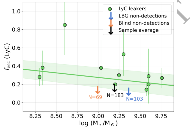
Figure 9. LyC f_{\text{esc}} as a function of stellar mass for candidate LyC leakers in our sample (green points), and stacked measurements from LBG selected (blue arrow), blind-selected galaxies (orange arrow) and the sample average (black arrow) in this study. The number of galaxies used in the stacking measurement are also given. We find a very weak correlation between f_{\text{esc}} and stellar mass, with a best-fit slope -0.10 \pm 0.02 (solid green line, uncertainty in shaded region). This dependence on stellar mass is stronger than the recently observed lack of correlation between the two quantities for a sample of low mass ( < 10^8 M_{\star} ) galaxies at 0.3 \leq z \leq 0.45 by Izotov et al. (2021), however the scatter is very large. We note that the stacked limits are not included when obtaining the best-fit relations in this study.
