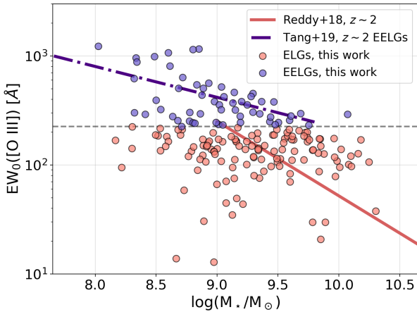
Figure 6. Distribution of EW_0([O\text{ III}]) and galaxy stellar mass derived for our sample of galaxies using SED fitting. Shown for comparison are the best-fit relations derived between the two quantities for relatively massive star-forming galaxies at z \sim 2 by Reddy et al. (2018) (red solid line) from the MOSDEF survey and extreme emission line galaxies (EELGs) at z \sim 2 by Tang et al. (2019) (blue dot-dashed line), where the black dashed line marks EW_0([O\text{ III}]) > 225\text{Å} , used by Tang et al. (2019) to classify galaxies as EELGs. The normalisation of the best-fit relations have not been altered. Galaxies from our sample that would be considered as normal emission line galaxies (ELGs) are shown as red points, and those considered as EELGs are shown using blue points. The distribution of our SED derived measurements (and the scatter) are broadly consistent with spectroscopic measurements at lower redshifts.
