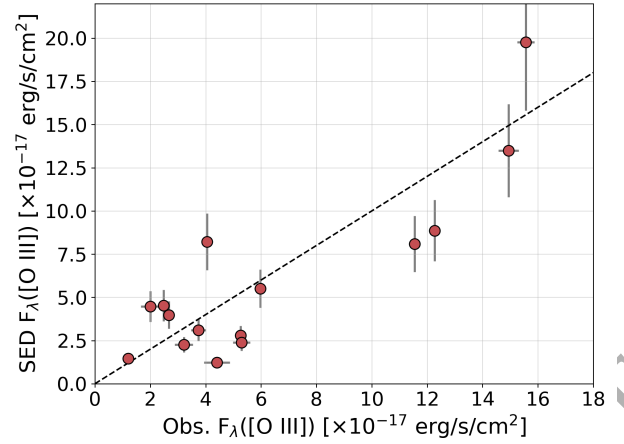
Figure 7. Comparison of [O III] + H \beta line fluxes measured from the best-fit SED and K -band excess and the observed line fluxes from NIR spectra. From the limited number of galaxies in our sample that have observed line fluxes from Cullen et al. (2021), we can conclude that our method of estimating line fluxes from K -band excess works reasonably well.
