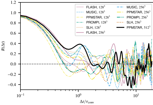
Fig. 4. Autocorrelation function R(\Delta t) of the convective velocity as a function of the time shift \Delta t in units of the convective turnover timescale \tau_{\text{conv}} . See Eq. (18) and the associated text in detail.
