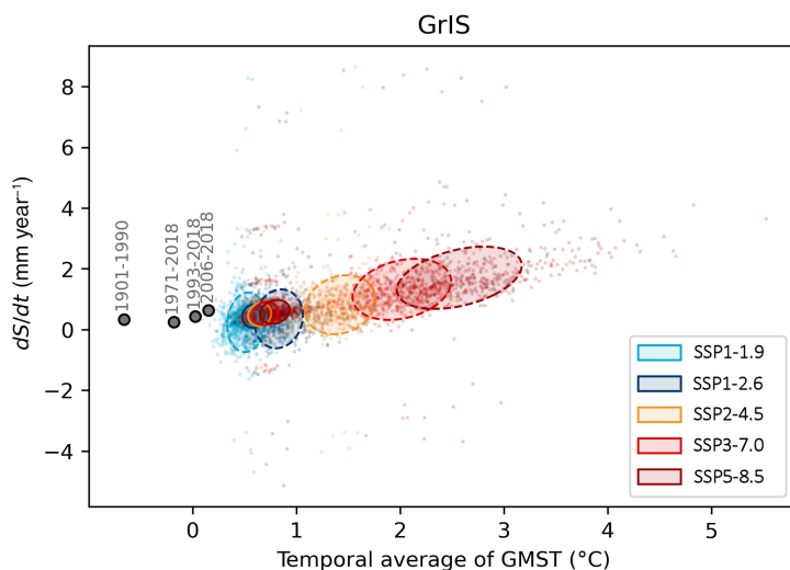
Figure 2. The transient sea level sensitivity (TSL) of the Greenland Ice Sheet (GrIS). The coloured dots show the sea level contribution of the ice sheet in \text{mm year}^{-1} for a given mean centennial temperature change based on CMIP6 Global Circulation Model forcing and temperature change for different Shared Socio-Economic Pathways (SSPs). Also shown as grey circles are observations and historical estimates of the ice sheet response. The x-axis shows the temporal average of global mean surface temperature (GMST). The y-label ( dS/dt ) is the change in mean global sea-surface height per unit time, in this case a year. It is apparent that over these timescales, the modelled response is a quasi-linear function of temperature.
