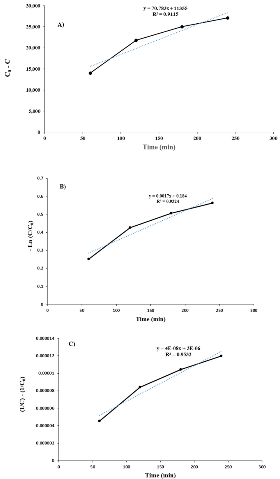
Figure 12. kinetics of sodium removal for real brine under optimal process conditions, (A): Zero-order (B): First-order (C): Second-order.
