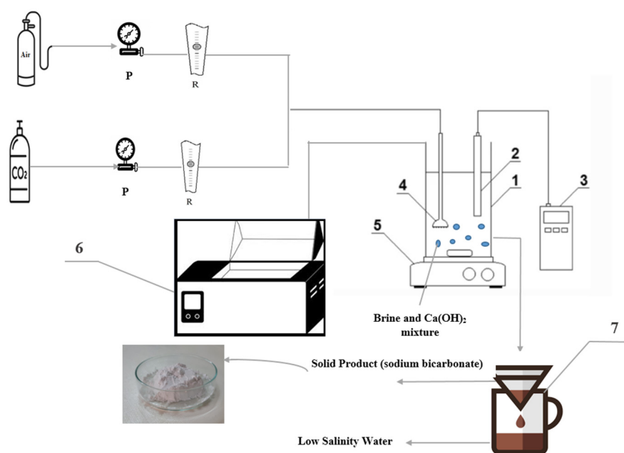
Figure 2. Experimental setup of modified Solvay process: 1—Double-walled Pyrex reactor, 2—pH electrode, 3—pH meter, 4—air stone, 5—magnetic stirrer, 6—water bath, 7—Filter, P—pressure gauge, R—rotameter.
