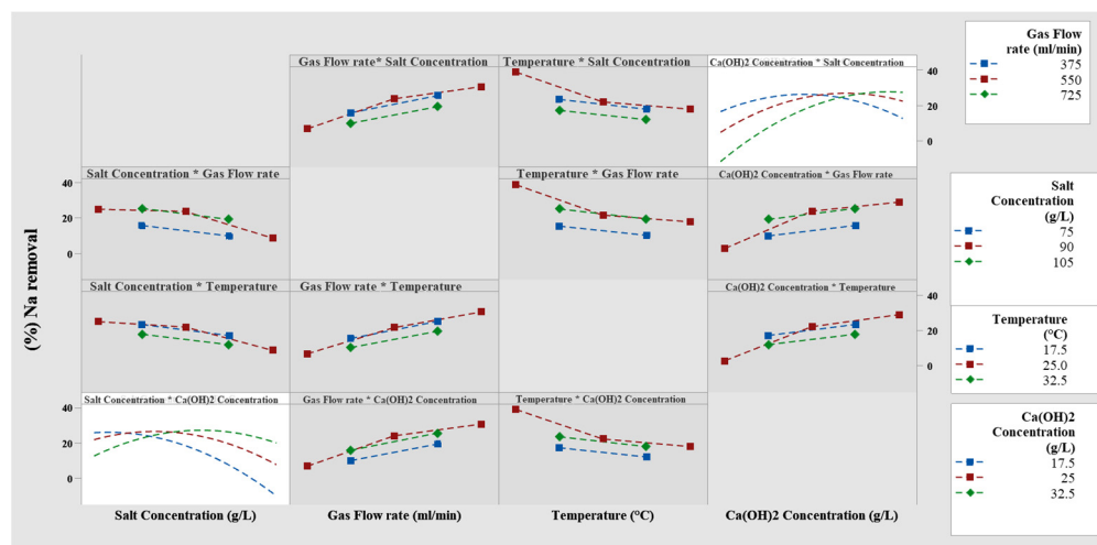
Figure 7. Charts of the effect of interaction between factors in sodium removal (%).
