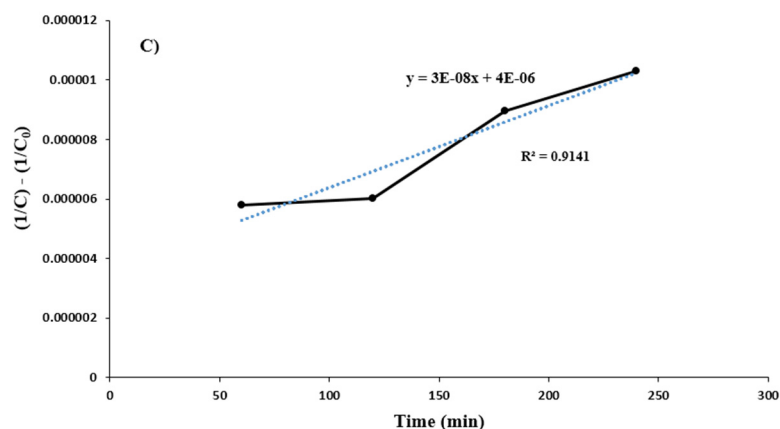
Figure 11. kinetics of sodium removal from synthetic brine under optimal process conditions, (A): Zero-order (B): First-order (C): Second-order.
