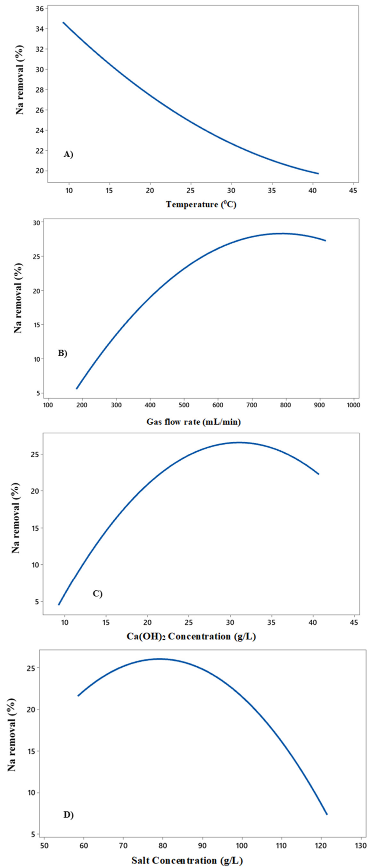
Figure 5. Linear regression of sodium removal (%) at temperatures of 10 °C to 40 °C (A), different gas flow rates (B), various calcium hydroxide concentration (C), and different sodium chloride salt concentration (D).
