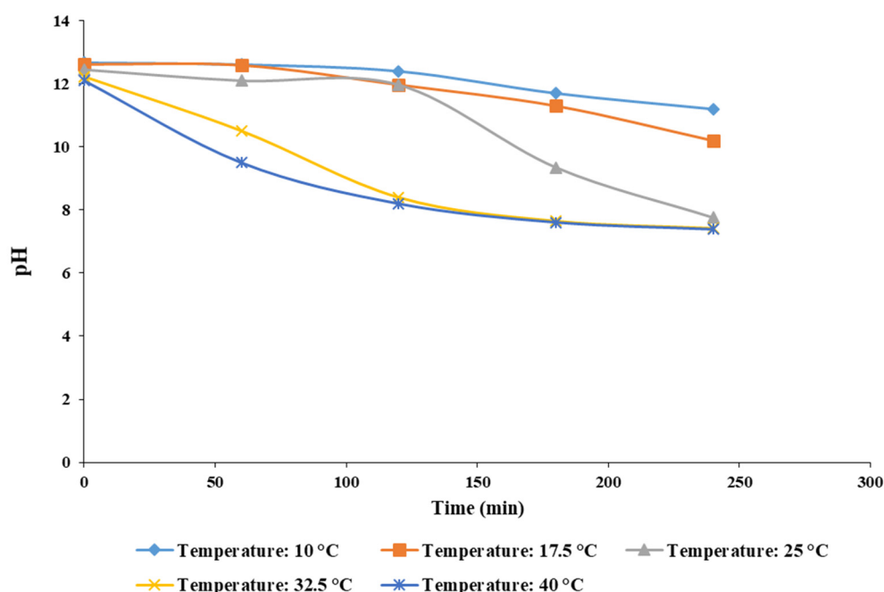
Figure 6. The effect of temperature on pH during different reaction times.
