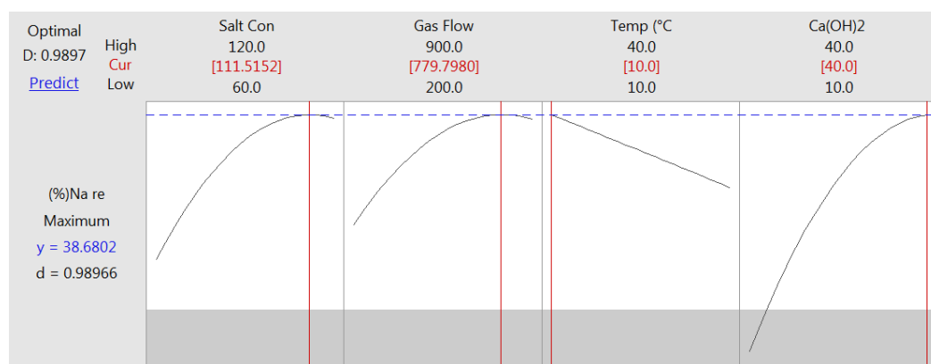
Figure 9. Chart of optimization of operational variables for sodium removal.
