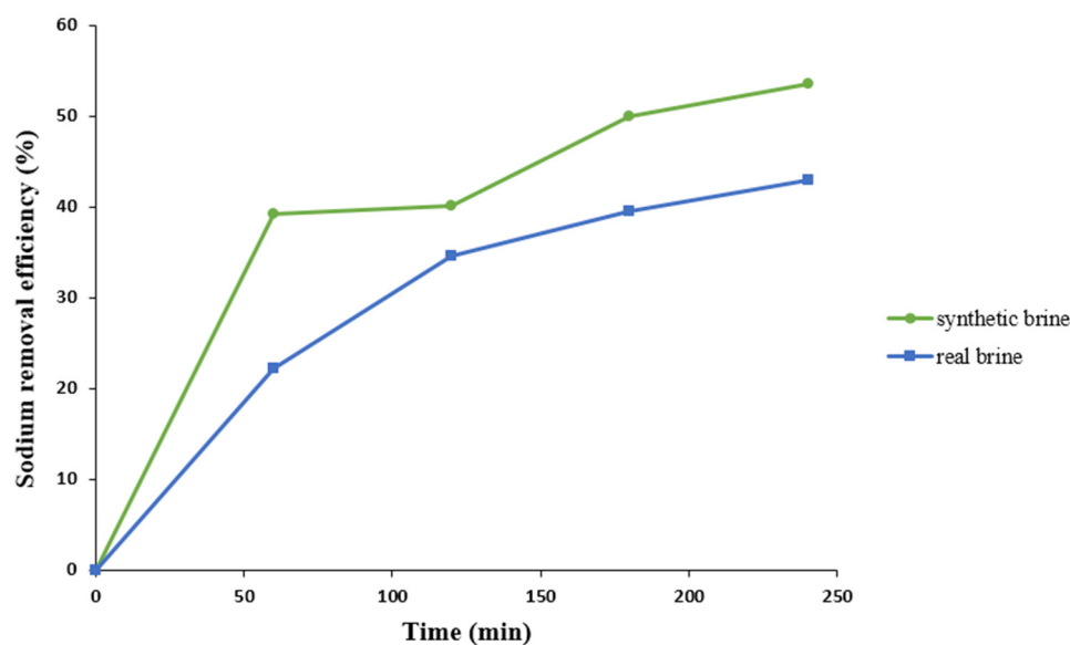
Figure 10. sodium removal efficiency under gas optimal conditions (calcium hydroxide concentration 40 (g/L), sodium chloride concentration 111.5152 (g/L), temperature 10 °C and gas flow rate 779.798 (mL/min) in synthetic and real brine.
