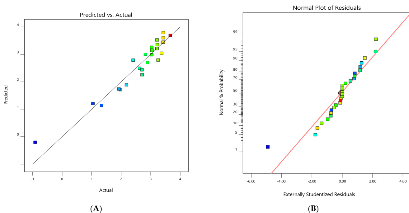
Figure 4. Experimental data vs. the statistical model's expected data (A) and normal residuals' normal probability (B).
