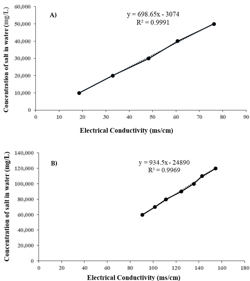
Figure 3. Calibration chart for conversion of electrical conductivity to total soluble solids in (A) 10,000 to 50,000 (mg/L). (B) 60,000 to 120,000 (mg/L).
