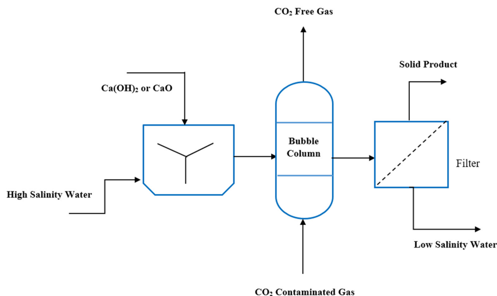
Figure 1. Scheme of the Solvay process based on calcium oxide.
