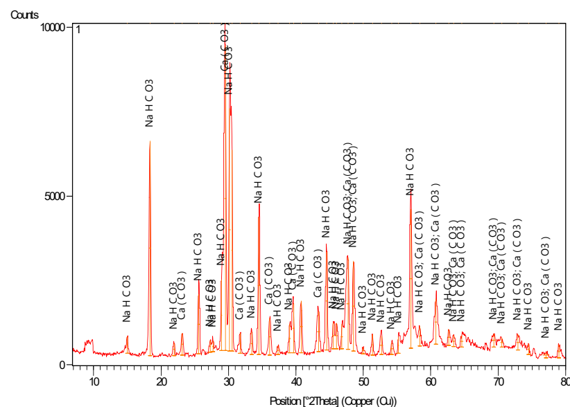
Figure 13. X-ray diffraction spectroscopy analysis of solid sodium bicarbonate product.
