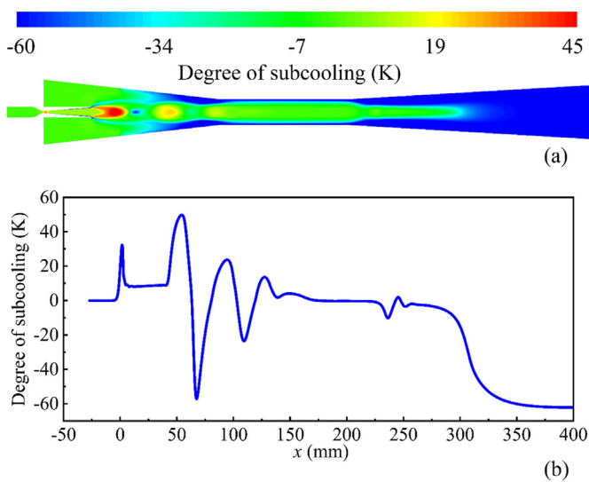
Fig. 8. Degree of subcooling within a steam ejector.
