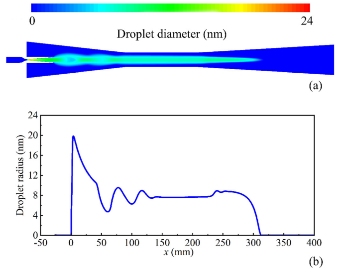
Fig. 10. Droplet diameter within a steam ejector.
