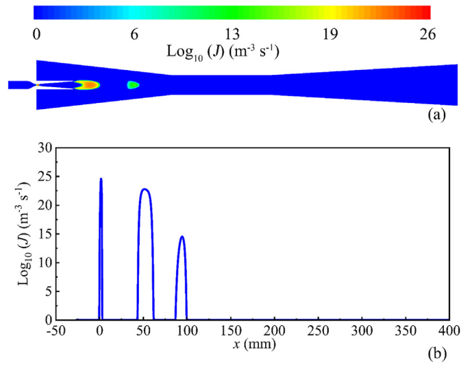
Fig. 9. Nucleation rate within a steam ejector.
