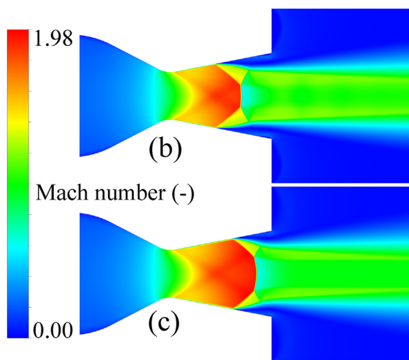
Fig. 5. The Hunter's nozzle [50] results: pressure comparison between the simulations and experiments (a), Mach number contours using k-\omega SST model (b) and k-\epsilon standard model (c).
