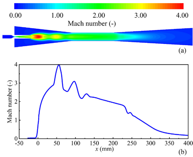
Fig. 7. Mach numbers within a steam ejector.
