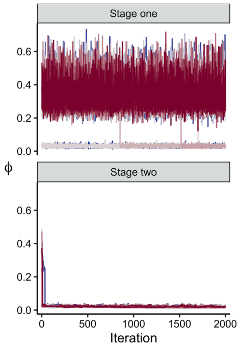
Fig. 2 Top: Stage one trace plot for \phi using the naive method. At any moment in time chains can jump to the spurious mode, which is an artefact of \hat{p}_1(\phi) . Bottom: Corresponding stage two trace plot. The stage two target has the same numerical instability, and because the stage one samples are the proposal distribution, all chains encounter the instability
