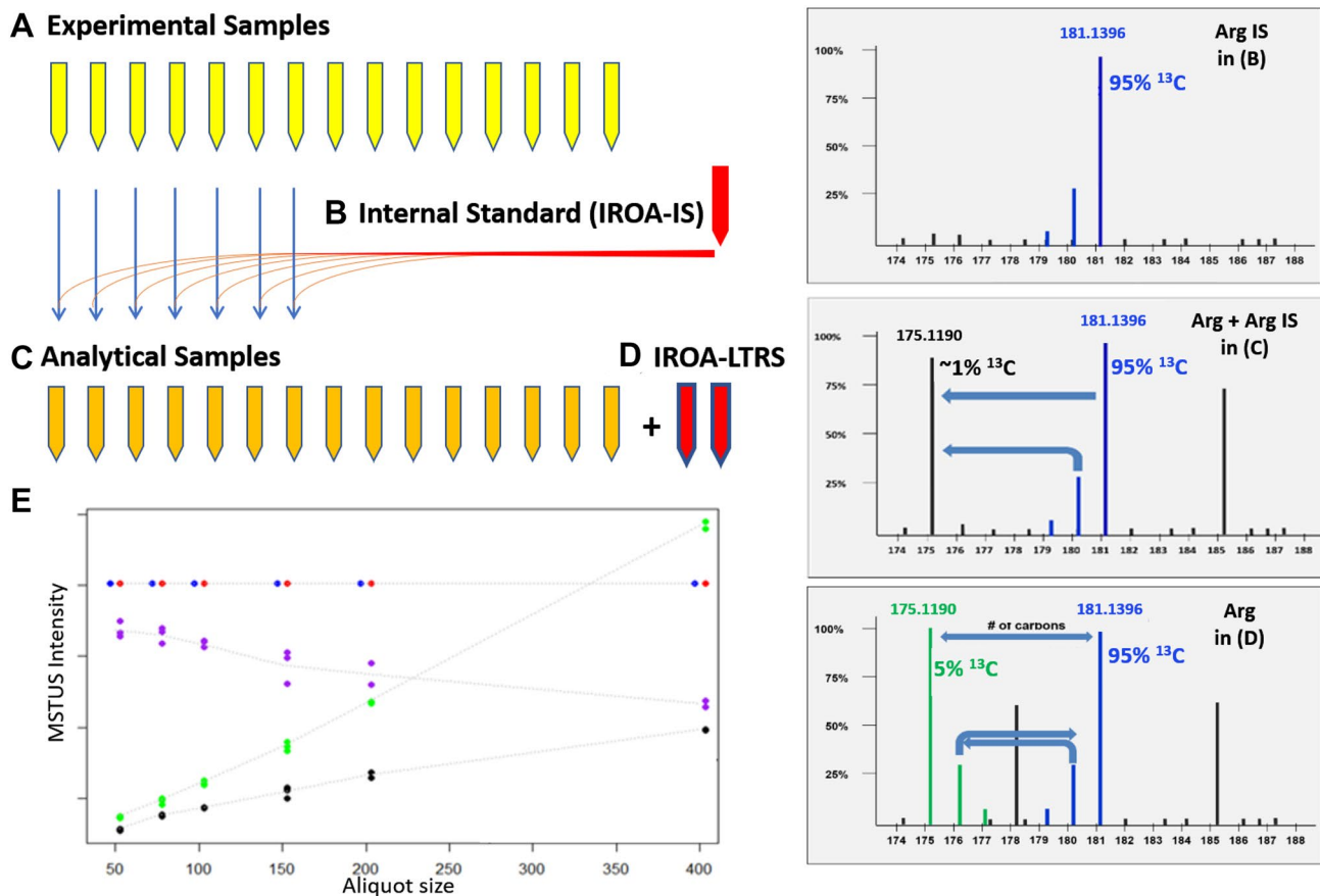
Fig. 4 The IROA TruQuant measurement system with the experimental samples A is spiked with the B internal standard (IROA-IS) to generate C analytical samples that are also paired with an D isotopically labeled Long Term Reference Standard (IROA-LTRS). Example mass spectra of an analytical sample C for arginine (Arg) with the
