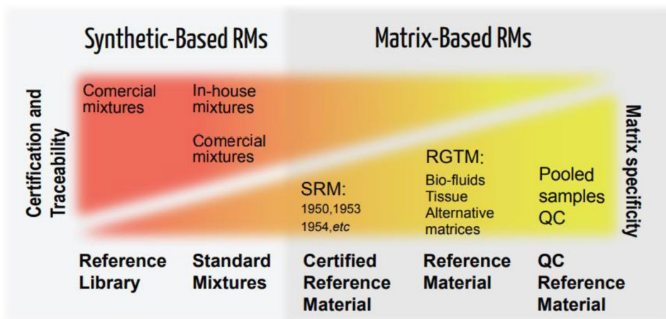
Fig. 1 Range of reference materials employed in the field of metabolomics and lipidomics. Gradient colors from yellow to red represent the inverse relationship between matrix specificity to the study samples and the metabolite traceability to certified standards. Each of
