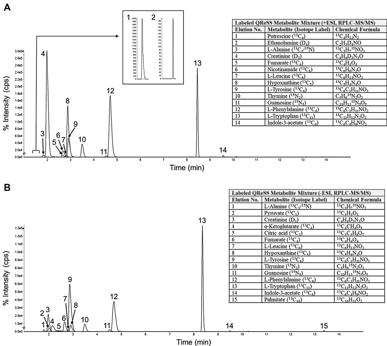
Fig. 3 Total ion chromatogram (TIC) of a matrix-free, combined QReSS mix measured by RPLC-MS (Phenomenex Kinetex F5 column, SCIEX TripleTOF® 6600 LC-MS/MS System). Acquisition
