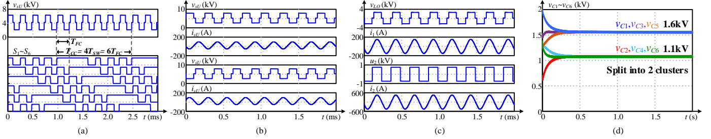
Fig. 6 Simulation results of n=6, m=2, L=3, N_h=2 as an unbalanced case with SM capacitor voltages splitting into 2 clusters for LLC-based MMDC. (a) Steady-state upper stack voltage and upper stack SM driving signals. (b) Steady-state voltages and currents of upper and lower stack. (c) Steady-state voltages and currents of input and output side of ac passive stage. (d) Dynamic SM capacitor voltages of upper stack.
