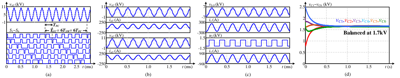
Fig. 8 Simulation results of n=6, m=0, L=7, N_h=1 as a balanced case for LLC-based MMDC. (a) Steady-state upper stack voltage and upper stack SM driving signals. (b) Steady-state voltages and currents of upper and lower stack. (c) Steady-state voltages and currents of input and output side of ac passive stage. (d) Dynamic SM capacitor voltages of upper stack.
