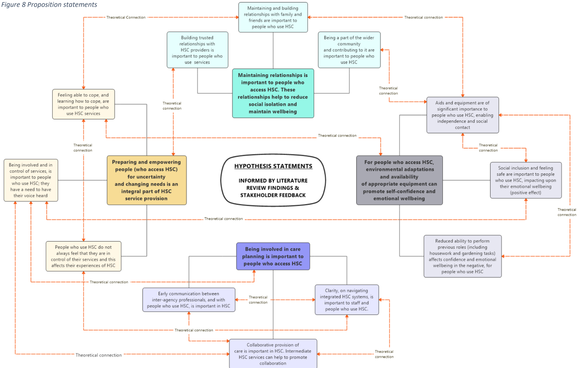
Figure 8 Proposition statements
