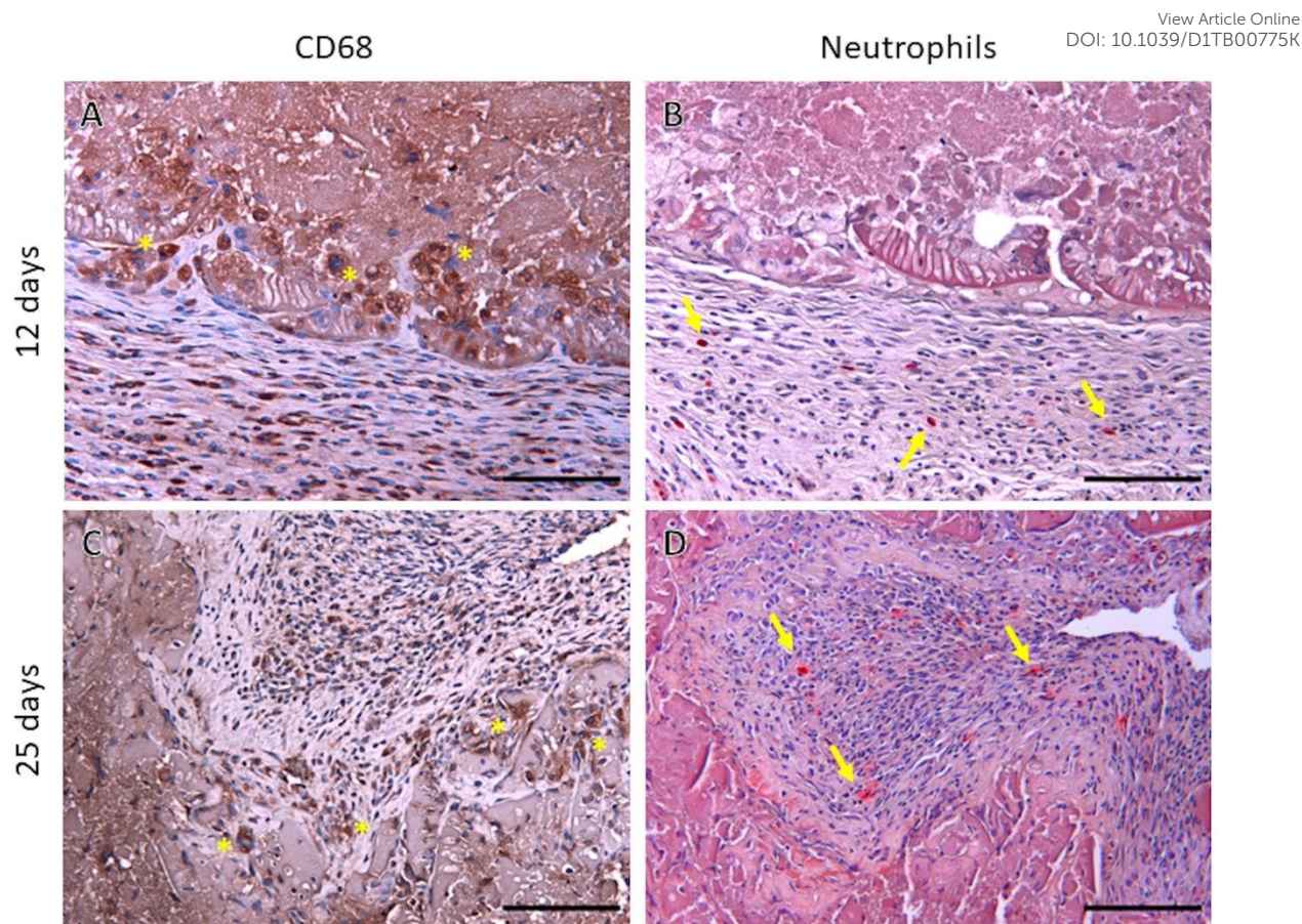
Figure 8. Paraffin sections from oligo-His-PLGA scaffolds were analysed by histology using immunohistochemistry with anti CD68 antibody (A, C) or stained for neutrophil (chloroacetate esterase staining) (B, D). Asterisks indicate engulfing scaffold macrophages. Arrows indicate neutrophils (magnification x20). Scale bars= 100 \mu\text{m} .
