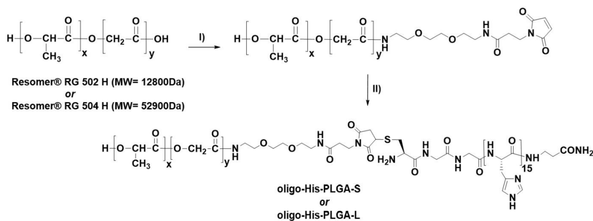
Figure 1. Schematic synthesis of oligo-His-PLGA-S and oligo-His-PLGA-L: I) (1-[Bis(dimethylamino)methylene]-1H-1,2,3-triazolo[4,5-b]pyridinium3-oxid hexafluorophosphate
