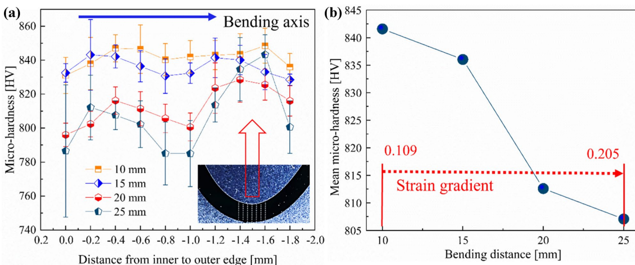
Fig. 3 a The hardness transition along the bending axis at different moving distances; b comparison of mean hardness under various conditions. The development of strain gradient owing to austenitising bending was plotted
