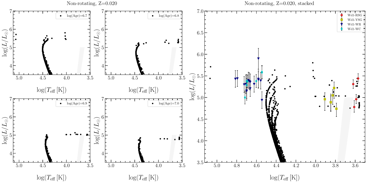
Figure 9. HRD of synthetic clusters with \log_{10}(\text{age}/\text{yr}) = 6.7, 6.8, 6.9, 7.0 , at Z=0.020 , each with 10,000 initial stars, without rotation. Left : Individual 10,000-star clusters considering instantaneous star formation. Right : Cluster of 40,000 initial stars combining (stacking) the stars from the four 10,000-star individual clusters on the left, corresponding to a star formation episode lasting 5 Myr.
