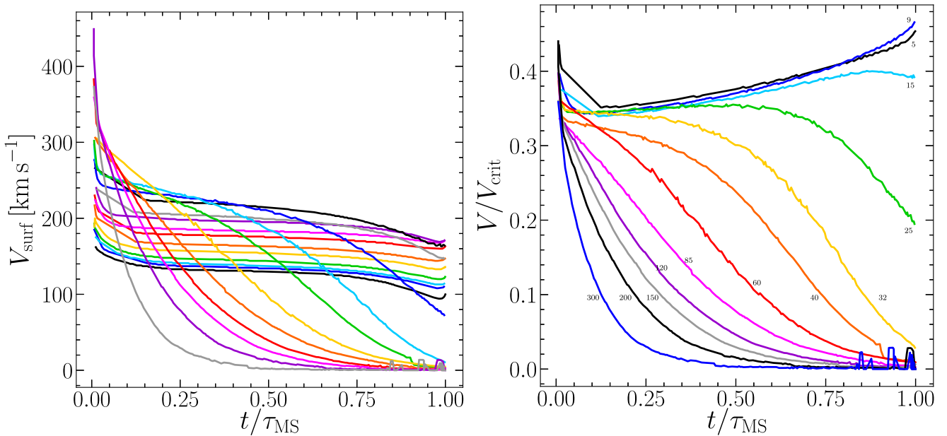
Figure 2. Velocity evolution of the rotating models at Z = 0.020 as a function of the MS lifetime. Left : surface velocity. Stars from 1.7 (lowest track at t/\tau_{\text{MS}} = 0 ) to 300 M_{\odot} . Right : ratio V/V_{\text{crit}} of selected massive star models.
