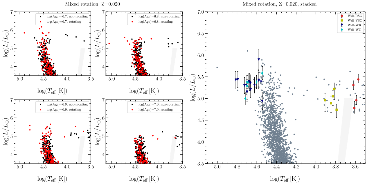
Figure 11. HRD of synthetic clusters of \log(\text{age}/\text{yr}) 6.7, 6.8, 6.9, 7.0, at Z = 0.020 , each containing 10 000 initial stars with mixed rotation: 7000 without rotation (black dots) and 3000 with rotation (red dots). We added Gaussian noise on L and T_{\text{eff}} to simulate observed stars ( \sigma_L = 0.2 dex, \sigma_{T_{\text{eff}}} = 0.05 dex). Left: Individual 10 000-star clusters considering instantaneous (or very brief) star formation. Right: Cluster of 40 000 initial stars combining the stars from the four 10 000-star individual clusters on the left, corresponding to a star formation episode lasting 5 Myr.
