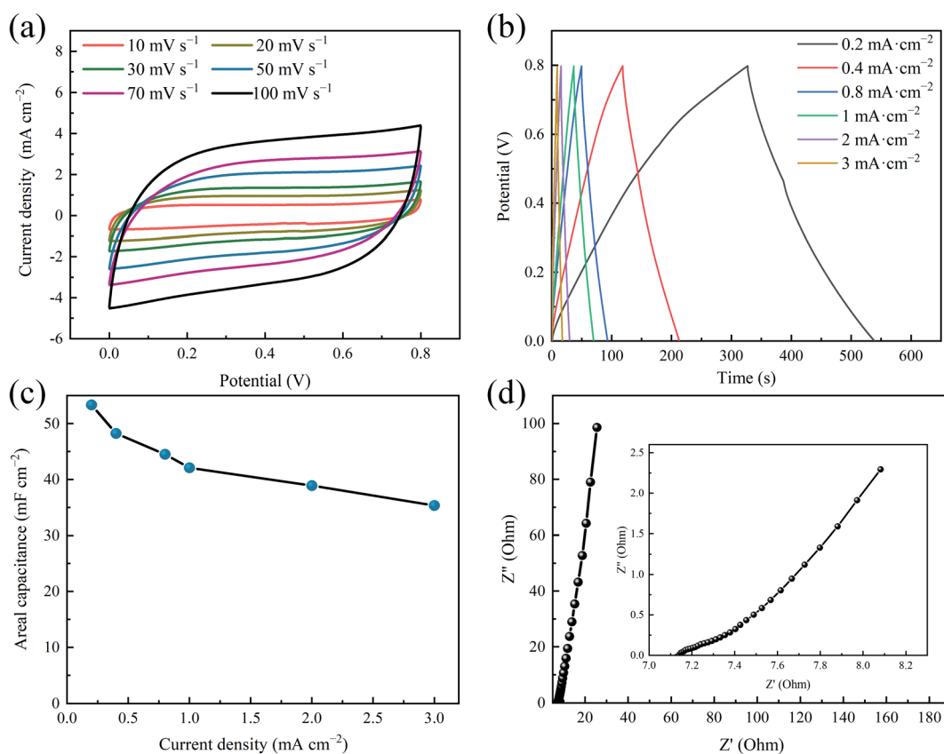
Fig. 5 Electrochemical characterization of the SC based on TiC NTA electrode. (a) CV curves at different scan rates ranging from 10 to 100 mV s -1 ; (b) GCD curves at various current densities ranging from 0.2 to 3 mA cm -2 ; (c) specific capacitances at various current densities; (d) Nyquist plots of the flexible SC, the inset shows the details in the high-frequency range.
