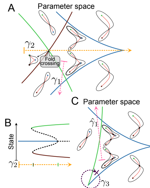
Figure 10: Families with a dual cusp. A and C. Bifurcation sets. Two landscape families with a dual cusp. The solid lines show the bifurcation set with the colour of the line corresponding to the attractor involved in the fold bifurcation. The dashed arrows illustrate paths in parameter space. A. The region where there are three attractors is bounded by a dual cusp and fold curves with crossings. The crossings that can occur are highly constrained [2]. Path \gamma_1 corresponds to a French Flag landscape. B. Symmetry breaking. This bifurcation diagram corresponds to the path \gamma_2 in A. It is the dual cusp version of the pitchfork bifurcation that occurs in the standard cusp. Like the pitchfork it is not generic but in the exceptional case where there is a \mathbb{Z}_2 -symmetry such as when the system describes the behaviour of two identical cells it becomes generic and describes an interesting symmetry breaking bifurcation (see [24] for an example). C. A three attractor region bounded by a dual and standard cusp. Path \gamma_1 corresponds to the French Flag landscape. Path \gamma_3 corresponds to the cusp smooth state swap of the green and blue attractors.
