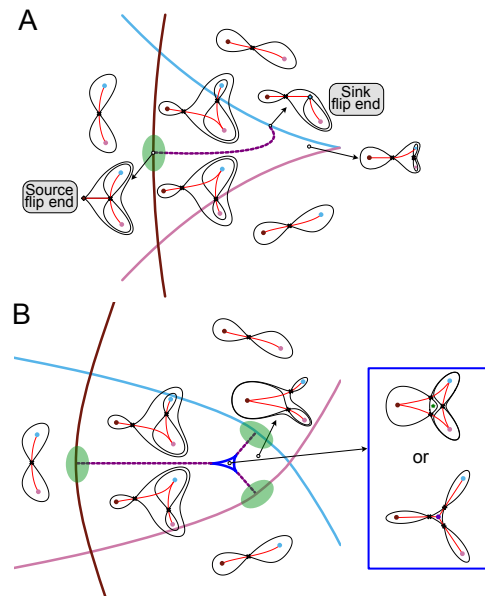
Figure 12: Families with flip curves. A,B. Bifurcation sets. The bifurcation sets for two landscape families: the solid lines indicate fold curves and the dashed lines are flip curves. The colour of the fold line corresponds to the attractor involved in the fold bifurcation. Examples of landscapes in the family are sketched. Both families contain the flip landscape in the areas marked in green. A. One flip with a cusp. The two attractors connected to the sink saddle can undergo a cusp bifurcation. B. With no cusps. This family contains three instances of the flip landscape. The region enclosed by the blue deltoid corresponds to landscapes with an extra pair of critical points: a saddle and either a repeller or an attractor (as shown in the blue box). This family is part of the compactified elliptic umbilic catastrophe.
