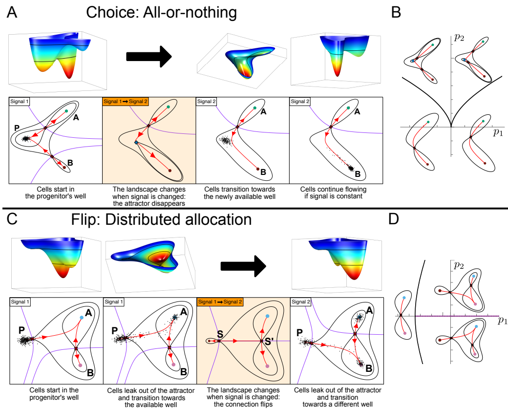
Figure 3: Binary decisions. A. Binary choice landscape. In the starting condition, Signal 1, cells are in a progenitor state corresponding to the middle basin of the landscape. Exposure to Signal 2 results in the disappearance of the central basin and the bottom ridge and cells transition into State B following the slopes of the new landscape. B. Two parameters p_1 and p_2 govern the landscape in A . Bifurcations occur when these parameters are on the black curves in p_1, p_2 -space. Crossing one curve results in cells transitioning to A ; crossing the other cells transition to B . C. Binary flip landscape. Cells start in the progenitor state P which corresponds to a shallow basin. Noise is sufficient for cells to transition into the more committed states and they follow the escape route (red) towards state A when exposed to Signal 1. In response to Signal 2 the escape route flips towards B and cells transition towards B . D. The landscape in C is also governed by two parameters. The progenitor attractor is destroyed when the parameters are on the black curve and the flip occurs when the parameters are on the purple curve.
