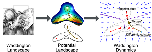
Figure 1: From Waddington's landscapes to Waddington dynamics. The classic picture of a Waddington Landscape (left) can be formalised using a potential function (middle). Nevertheless, to capture the full behaviour of the system the complete Waddington dynamics are needed (right). The dynamics describe the trajectories cells take between different states.
