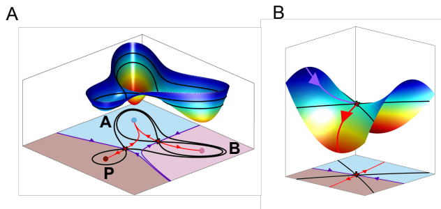
Figure 2: Two Dimensional Landscapes. A. System with three attractors and two saddles. The purple curves are the separatrices or stable manifolds of the saddles, the red curves are the unstable manifolds (if time is run backwards points on these converge to the saddle). Points on each unstable manifold converge to two attractors and the stable manifolds divide the phase space into three basins, one for each attractor. Level curves for the saddles are indicated in black. B. Saddle Point. The dynamics near a saddle point. The stable (purple) and unstable (red) manifolds are shown.
