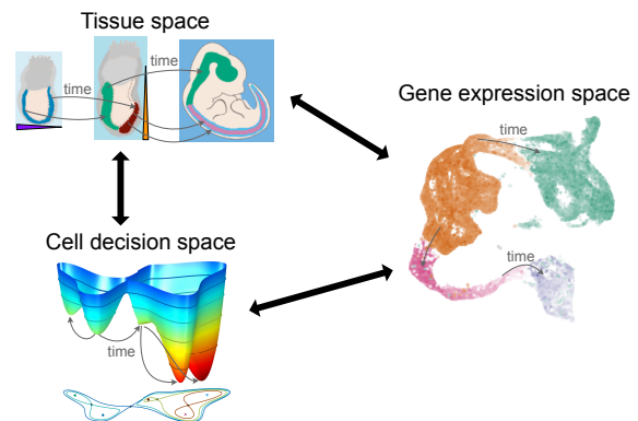
Figure 13: Three developmental spaces. A developing cell can be followed through three distinct spaces. The location of a cell in tissue space gives the coordinates of a cell in a developing embryo and indicates the signaling environment to which it is exposed. The same cell can also be represented in gene expression space by its molecular identity. In addition, the cell occupies a position within cell decision space . This is the location in a Waddington dynamics landscape, which represents its cell fate and describes the decision making process. The goal is to be able to link cells in these three spaces and to map how a cell moves through them over time.
