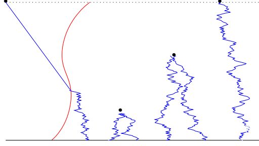
FIG 3. The exit measure can be transported by ballistic motion to the halfline (-\infty, g(t)) \times \{t\} .
