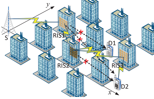
Fig. 2. Simulation environment.
