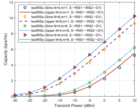
Fig. 3. Ergodic capacity vs transmit power with different N under different channels.
