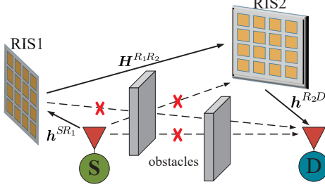
Fig. 1. Multiple RIS-assisted communication system with two RISs.
