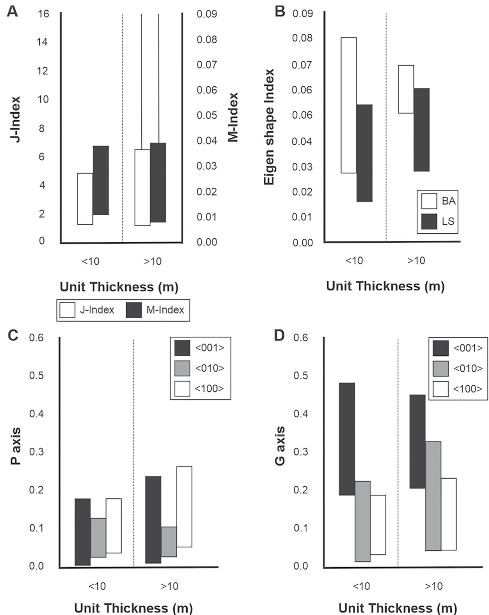
Figure 11. Calculated CPO indices compared against calculated crystal settling magma body unit thickness (Equation 4). (a) J-Index (here defined as low = 1.4–1.8, low-medium 1.8–3.0, medium = 2.4–5.0, medium-strong = 4.0–12.0, and strong >12.0) and M-Index (0 = random 1 = a single crystal); (b) Eigenvalue shape indices which range from 0 to 1 (0 = A or S and 1 = B or L). The BA-Index range for calculated magma bodies is observed to be more restricted for those >10 m; (c) lineation strengths (0.1–0.3 = weak, 0.3–0.5 = moderate, and >0.5 = strong) between the different crystallographic axes; and (d) foliation strengths for the different crystallographic axes (0.1–0.3 = weak, 0.3–0.5 = moderate, and >0.5 = strong). Between the lineation and foliation strengths foliation within the <001> axis is observed to range from weak to moderate, while all other axes show weak to no CPO.
