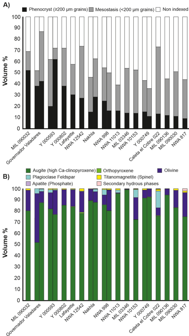
Figure 3. Modal mineralogy of the nakhrites from electron backscatter diffraction (EBSD) data. (a) Area percent of phenocrysts ( \geq 200 \mu\text{m} crystals), mesostasis material ( < 200 \mu\text{m} crystals), and non-indexed material (mainly glass and fractures but can also consist of holes and amorphous material). (b) Area percent of all indexed phases in EBSD data that is, this is for both phenocryst and mesostasis phases. (See Supporting Information S1 for data in table version).
