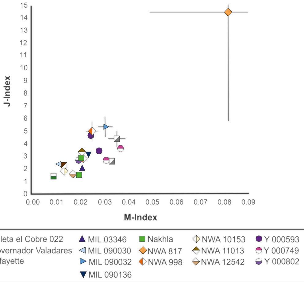
Figure 7. M-Index and J-Index values for the nakhilites. Caleta el Cobre 022 exhibits the lowest J-Index and M-Index values, while the highest observed J-Index and M-Index values, for NWA 817, are interpreted to be a function of the smaller data set size ( n_{\text{MTEX}} = 43 crystals).
