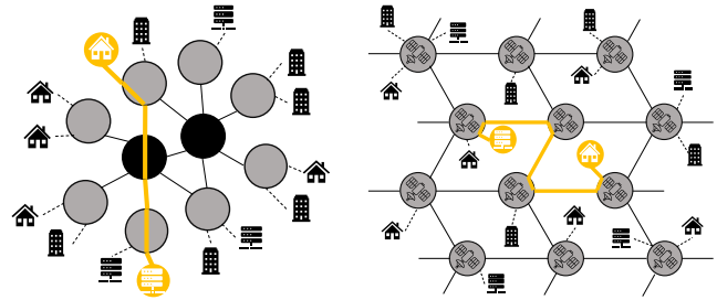
(a) Traditional network topology. (b) LEO Internet topology.
