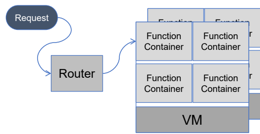
Fig. 6: High-level overview of typical FaaS platforms: Requests are sent to a router component responsible for load balancing and authorization before being sent to a function container (either an actual Linux container [96] or a microVM [97]) for execution on a VM or physical machine.
