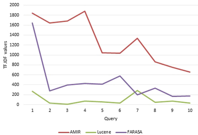
Fig. 6. The calculated TF.IDF values achieved by AMIR, LUCENE, and FARASA.
