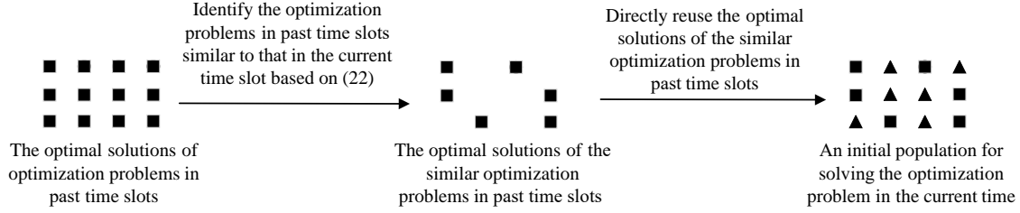
Fig. 4. Overall process of LETO to generate an initial population in the current time slot, where ■ represents the optimal solution of the optimization problem in past time slots and ▲ represents the randomly generated solution.
