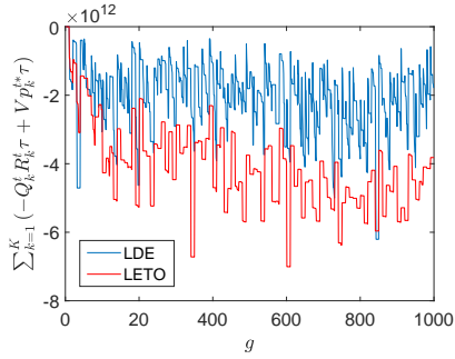
Fig. 8. Dynamics of the objective values of LETO and LDE when N = 25 and K = 30 , where the maximum value of g is equal to g_{\max} * t_{\max} (i.e., 1,000).
