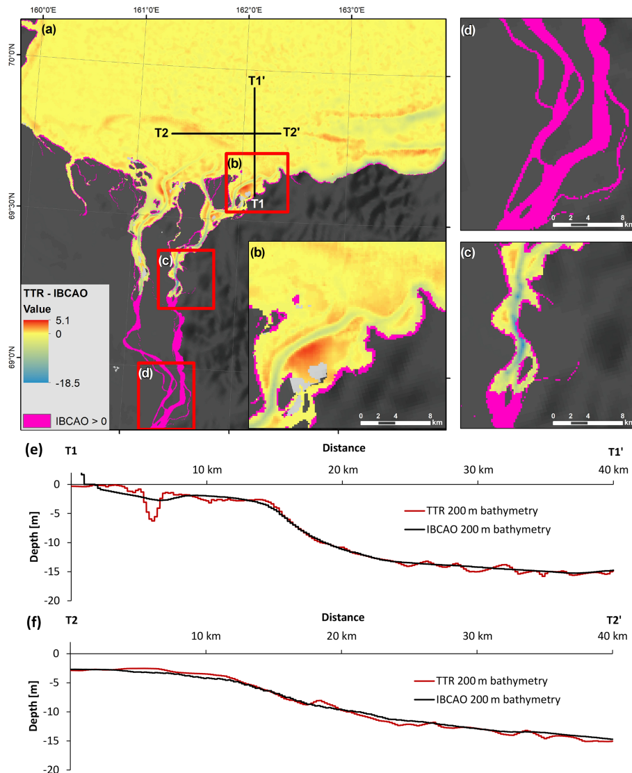
Figure 9. Depth difference map for the TTR 200 bathymetry model and the IBCAO v4 200 m bathymetry data set in the Kolyma Gulf region (TTR 200 minus IBCAO v4). Purple zones show areas where the IBCAO v4 incorrectly provides values above sea level. Reddish areas depict zones where the IBCAO v4 overestimates the depth in comparison to the TTR 200 . Blueish areas show zones where the IBCAO v4 has lower water depths than the TTR 200 . The highest positive value (5.1 m, red) means that the IBCAO v4 indicates a depth which is 5.1 m deeper than in the TTR 200 . Panels (e) and (f) show cross-sections deriving depth data from both data sets (TTR 200 in red and IBCAO v4 in black) in the near-shore zone, directly comparing the TTR 200 and the IBCAO v4 bathymetry model, indicating a generally good agreement between the two data sets with the exception of deep main river channels (e).
