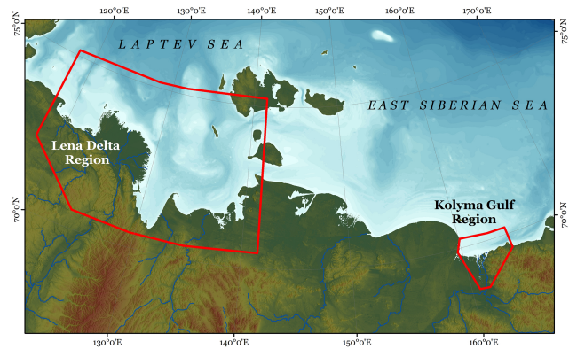
Figure 1. Study areas (red frames) of the Lena Delta and Kolyma Gulf regions. The background image is the IBCAO v4 200 m spatial resolution raster map (Jakobsson et al., 2020).
