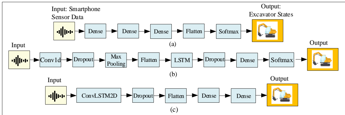
Figure 2: (a) DNN model architecture; (b) CNN-LSTM model architecture; (c) Conv-LSTM model architecture
