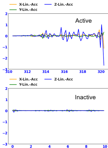
Figure 5: Sample of linear accelerometer data in x, y and z axis for active and inactive states
