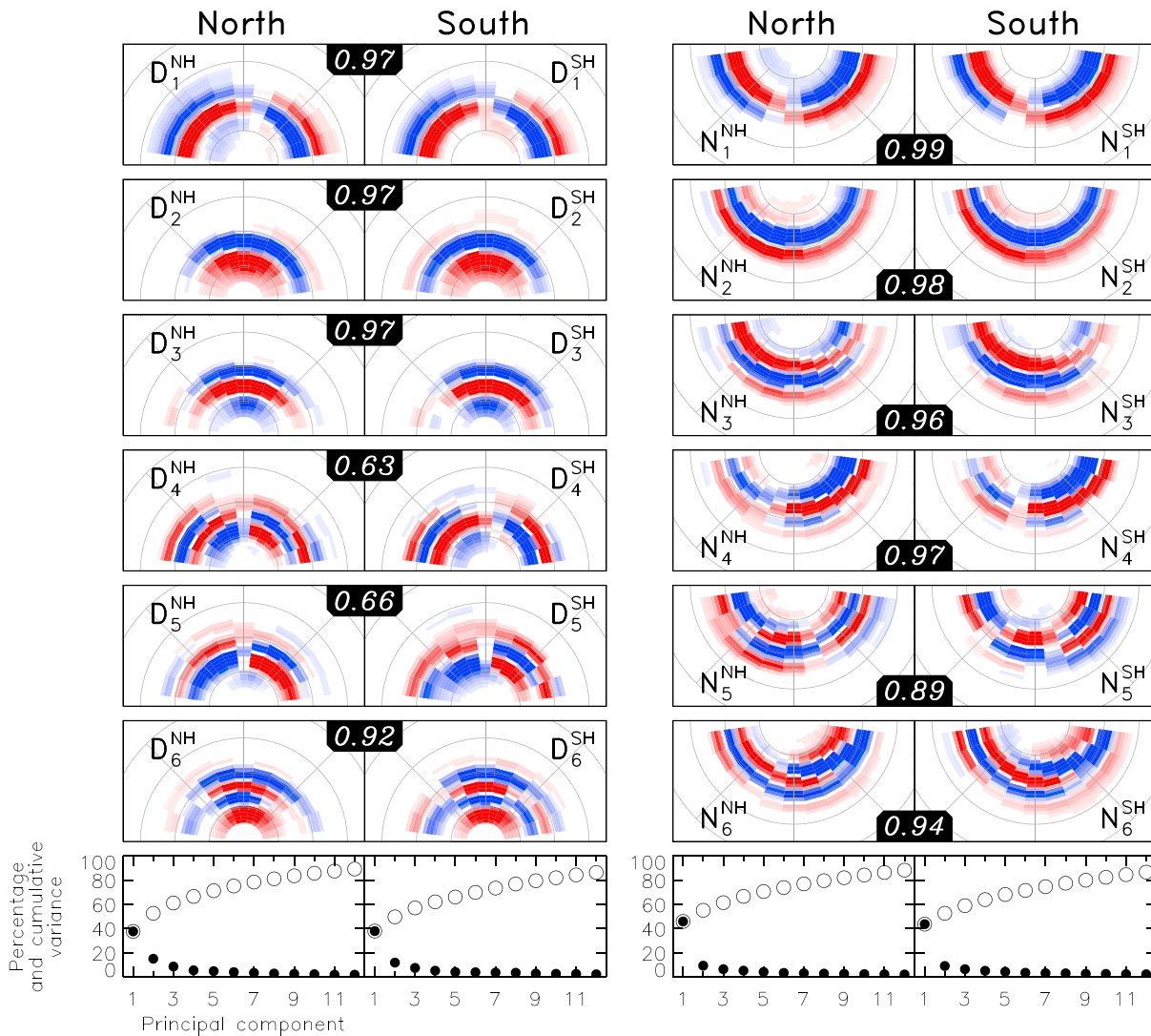
Figure 1. The first six eigenFACs for the dayside and nightside portions of the Northern and Southern Hemispheres Active Magnetosphere and Planetary Electrodynamic Response Experiment field-aligned current distributions, for the years 2010 to 2016. Each panel is presented in a magnetic local time and magnetic latitude frame, where magnetic latitudes are scaled such that the boundary between R1 and R2 FACs occurs at 70° (see text for details). Each north-south pair of eigenFACs has a coefficient of correlation quantifying their similarity. Bottom panels show the variance in the FACs explained by the first 12 eigenFACs. FAC = field-aligned current.
