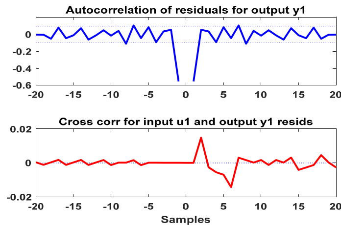
Figure 6. Model residual.
