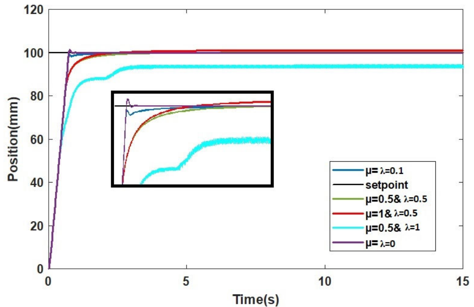
Figure 14. Step response of the system with different values of \mu and \lambda .
