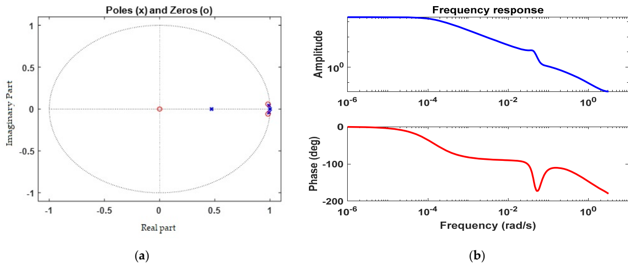
Figure 5. (a) Poles and zeroes; (b) frequency response.
