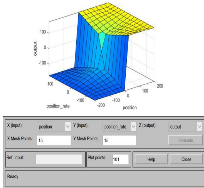
Figure 10. The surface viewer of the fuzzy.
