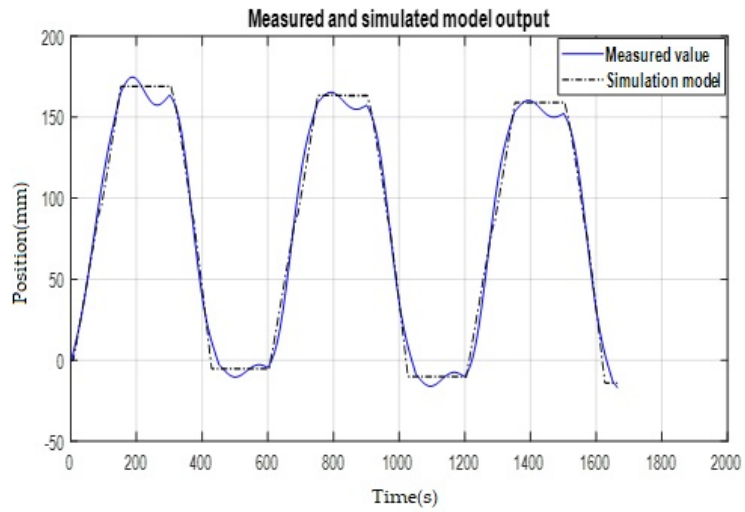
Figure 4. The measured and simulated model output.
