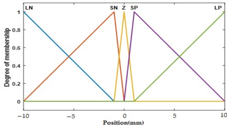
Figure 9. Inputs and output membership functions.
