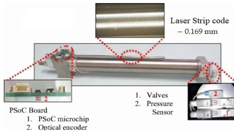
Figure 2. The pneumatic cylinder and its parts.
