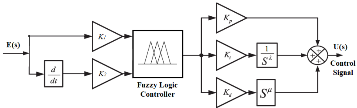
Figure 8. Block diagram of the fuzzy FOPID controller.
