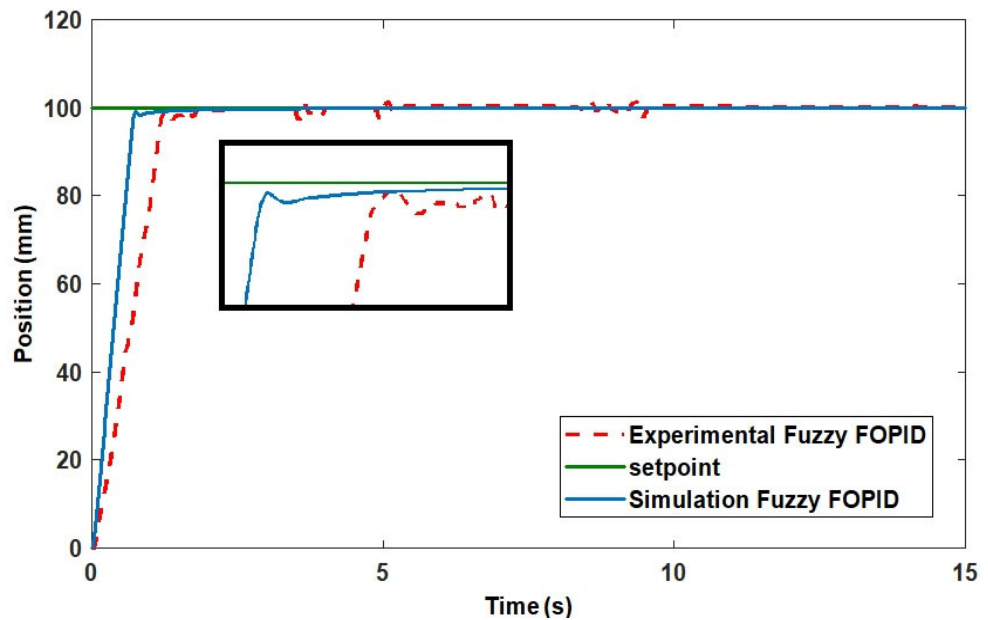
Figure 15. Fuzzy FOPID simulation and experimental performances.
