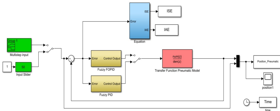
Figure 11. Simulink diagram for simulation.
