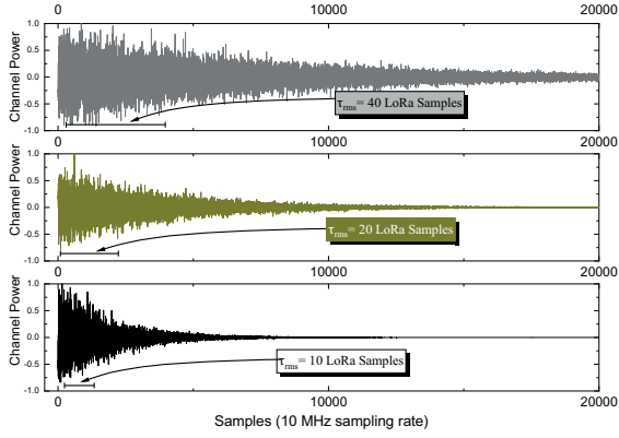
Fig. 3. Representation of the Rayleigh Fading Channels, shown here normalised to the maximum path. The RMS delay spread is defined in terms of LoRa samples to simplify the comparison with bin size.
