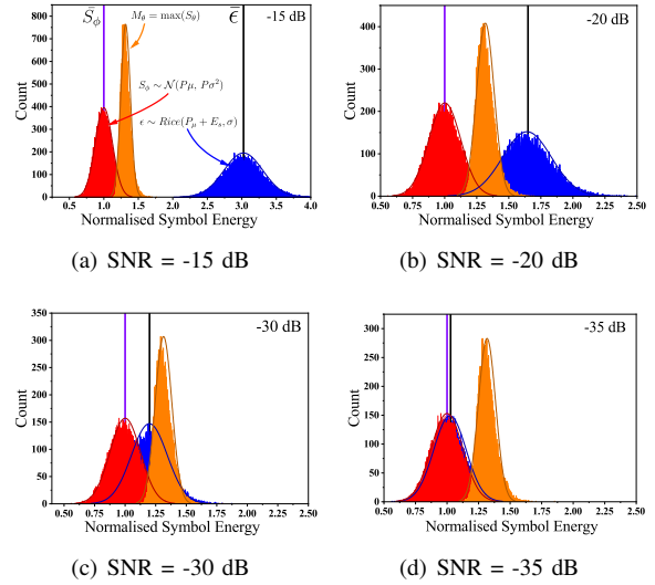
Fig. 4. Histograms: bin size = 64, 10 sample channel
