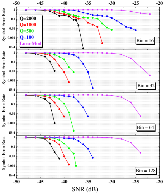
Fig. 8. Graph to show the improvement in performance with increasing Q at an SF=14. The channel used here is the 20 sample Rayleigh channel.
