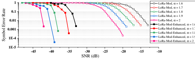
Fig. 10. Effect of Impulsive noise without clipping, Q=2000 , SF=14 , \text{Bin}=64 , 20-sample Rayleigh channel
