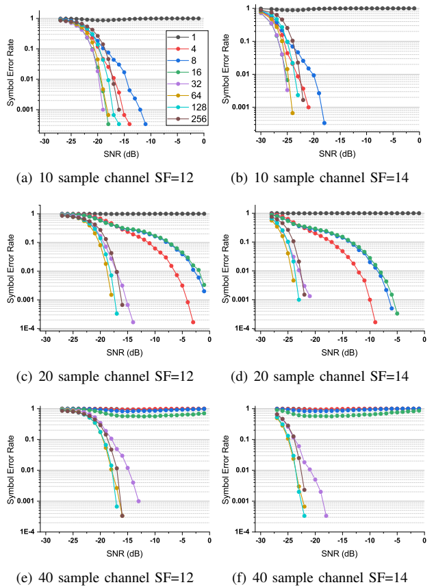
Fig. 5. Performance of LoRa-Mod : SNR Versus Symbol Error Rate as a function of superbin size, SF=12, 14, and various length Rayleigh channels.
