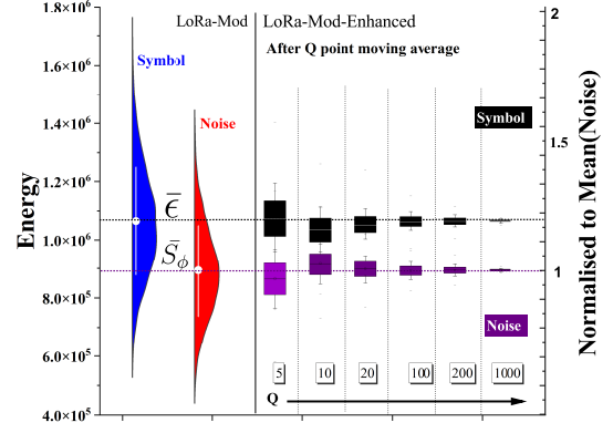
Fig. 6. Graphical demonstration of the working principle of Lora-Mod-Enhanced. In Lora-Mod, the Symbol energy is compared to the maximum energy of the remaining noise symbols. However, LoRa-Mod-Enhanced uses a Q -point moving average. The comparison is now between two distributions which are significantly narrowed, making error free communication in channels with extremely low SNRs (and significant multipath interference) possible.
