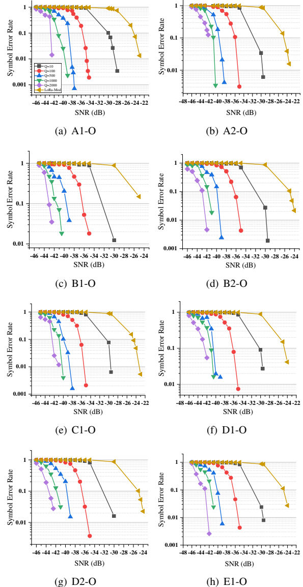
Fig. 13. SNR Versus Symbol Error Rate for SF=13, with 7,000 runs per simulation point. Impulsive noise is added ( \alpha = 1.7 ) with clipping ( M=1.3 ).
