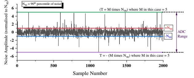
Fig. 9. Demonstration of the clipping technique. Shown here is a noise signal sampled from \alpha=1.8 distribution. In this case, M is chosen as 5, with sets a threshold of M \cdot N_{90} = 5 . The signal is normalised to the 90 th percentile of the absolute value of the measured noise signal, N_{90} .
