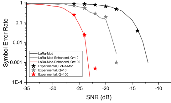
Fig. 15. Experimental versus Simulation results, where SF=10
