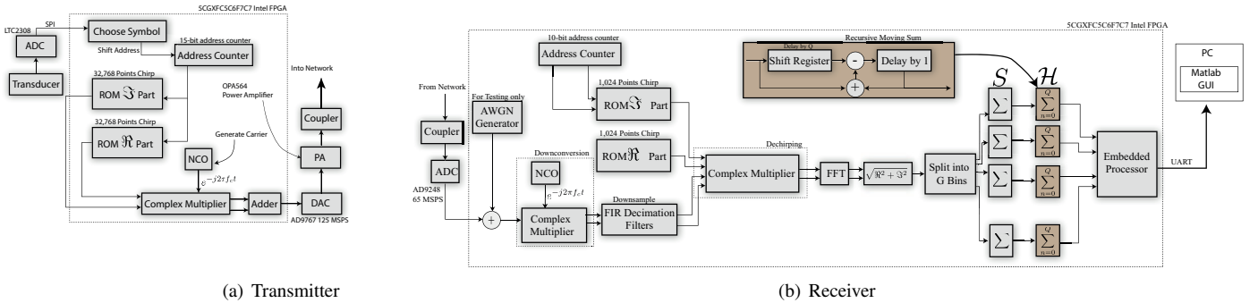
Fig. 14. FPGA based hardware architectures for the transmitter and receiver.
