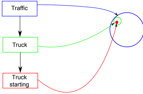
Figure 4: Spatial configuration of the Progressive Display (PD) based on the semantic hierarchical structure of the dataset
