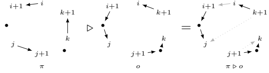
Figure 5: To show that \leq_\pi^\triangleright is transitive, we show first that (k, k+1) \notin \pi \triangleright o . Bullets indicate other potential items in \pi ; faded arrows indicate comparisons that may not be in \pi \triangleright o , but can be consistently added to it.
