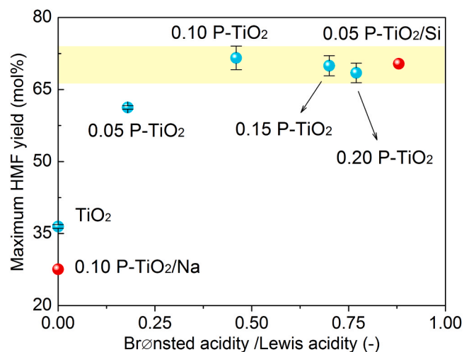
Fig. 8. Maximum HMF yield as a function of the ratio of Brønsted to Lewis acidity of the in-situ P-TiO 2 catalysts (determined by pyridine-IR as shown in Table 2).
