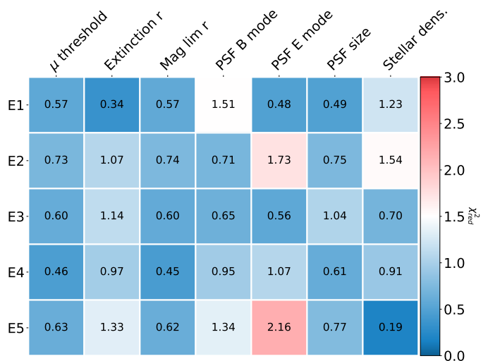
Fig. 6. Reduced \chi^2 for cross-correlations between the data’s tomographic pseudo E-modes and different systematics for a null detection. Here we show the systematics motivated in Sect. 4: object detection threshold ( \mu -threshold), extinction for the r -band, magnitude limit for the r -band, PSF ellipticities components in harmonic space (E/B-mode), the PSF size, and stellar overdensity from Gaia DR2 (Gaia Collaboration et al. 2018). The highest correlation occurs for the PSF E-mode in the fifth tomographic bin, this is shown in Fig. 7 to be subdominant to the cosmological signal given the estimated statistical error in this particular tomographic bin.
