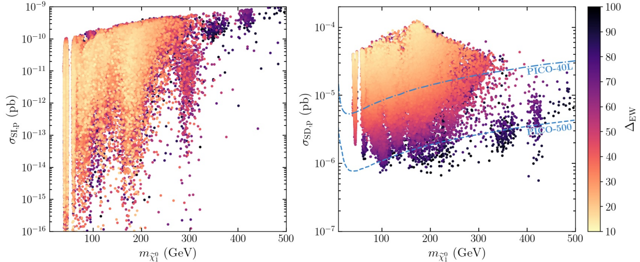
Figure 4: Right (left): The mass of the DM particle versus the spin-(in)dependent cross section \sigma_{\text{SD,p}} ( \sigma_{\text{SI,p}} ). The value of \Delta_{\text{EW}} is shown in color code. We also show the projected PICO-40L and PICO-500 central limits on \sigma_{\text{SD,p}} [141]. The points are ordered such that those with lower values of \Delta_{\text{EW}} lie on top of those with higher values.
