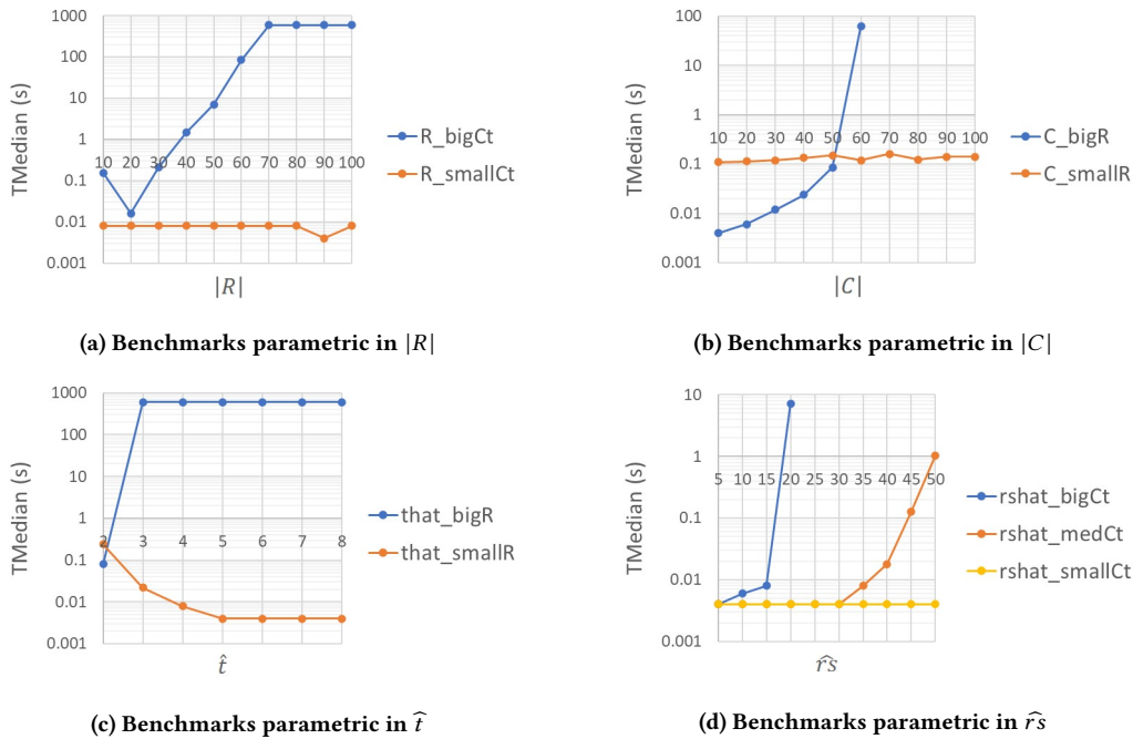
Figure 2: Performance of AQUA on the benchmarks of Table 2
