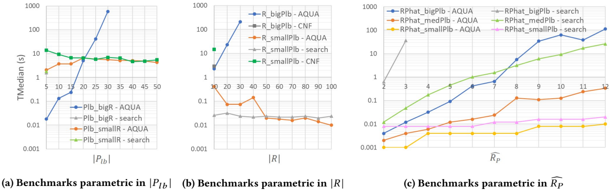
Figure 1: Performance of 2D-Opt-Search, 2D-Opt-CNF and AQUA on the benchmarks of Table 1
