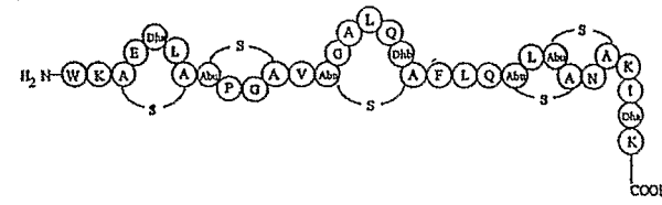
Subtilin
