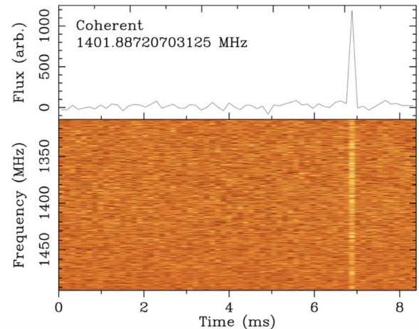
Figure 12. Detection of a giant pulse from the Crab Pulsar (B0521+21) using DSA-10. Top: incoherently summed and dedispersed pulse. Bottom: the same pulse, coherently summed and dedispersed. In each figure, the top panel is flux versus time, with flux normalized to the same arbitrary units, showing the summed power across frequency for each time step. The bottom panel of each figure is time versus frequency, showing the dedispersed pulse across the observing band during an approximately 8 ms time window. Channels affected by RFI have been blanked in the top figure. This RFI does not add coherently at the location of the Crab Pulsar, and as such they do not affect the bottom figure.
