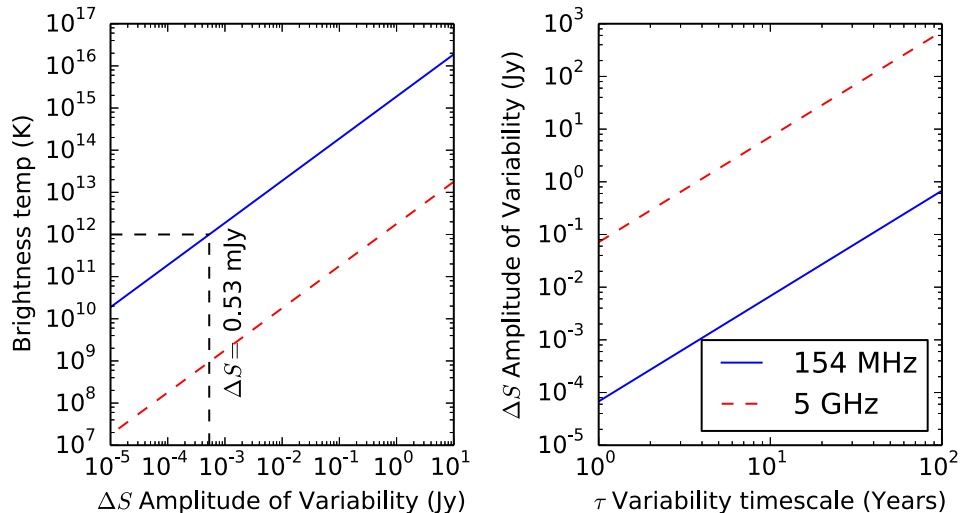
Figure 10. Left-hand panel: A plot of amplitude of variability ( \Delta S ) versus brightness temperature for a hypothetical source. We assume in this example that the source is at a distance of 10 Gpc and the variability time-scale is 2.8 yr. To not break the brightness temperature limit of 10^{12} K, the amplitude of variability ( \Delta S ) is restricted to be below 0.53 mJy (at 154 MHz). Right-hand panel: A plot of variability time-scale ( \tau ) versus amplitude of variability ( \Delta S ). In this case, we assume that T_b = 10^{12} K and we find that for typical variations of \Delta S = 0.5 Jy we require variability time-scales to be greater than \sim 100 yr (at 154 MHz). The comparison case of 5 GHz is shown with the red dashed line.
