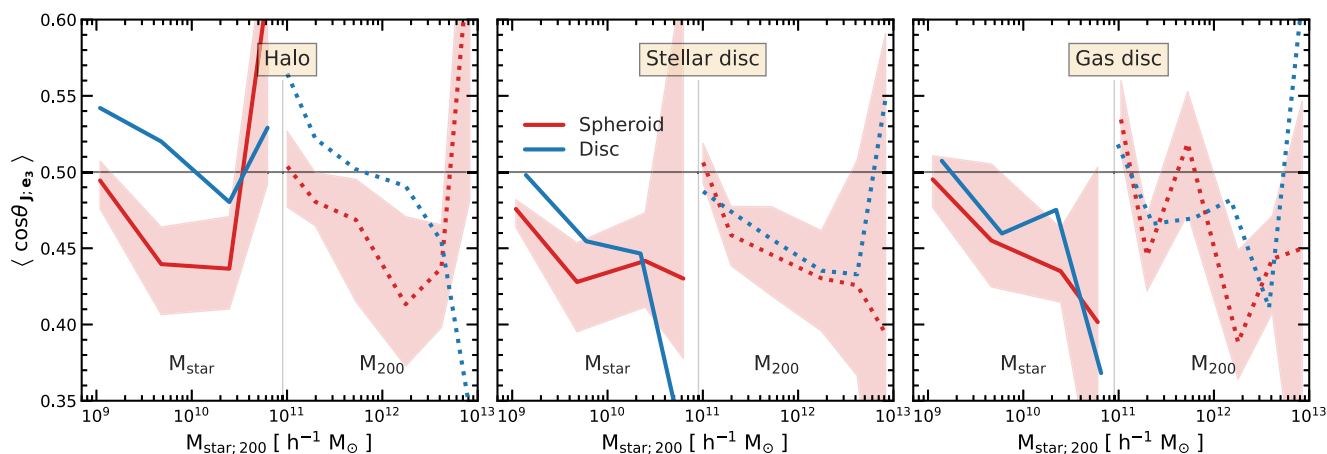
Figure 10. Spin–filament alignment for discs and spheroids: The plot shows the alignment as a function of both stellar mass (solid line) and halo mass (dotted line) for disc ( B/T < 0.58 , shown in blue) and spheroid ( B/T > 0.82 , shown in red) galaxies. The disc and spheroid samples were selected to contain a third of the galaxy population with respectively the lowest and highest bulge to total ratio. We only show the alignment with NEXUS+ filaments; however, this is very similar for Bisous filaments. The shaded region shows the uncertainty, as in Fig. 8.
