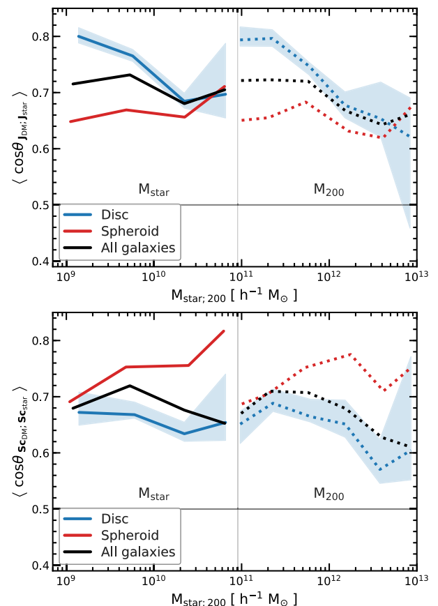
Figure 12. Galaxy–halo spin and shape alignment: The plot shows the median alignment angle of the spin (top panel) and of the minor axis (bottom panel) between haloes and their central galaxies. The alignment is shown as a function of both halo and stellar mass corresponding to all galaxies (black) as well as to two morphology-selected subsamples: discs (blue) and spheroids (red).
