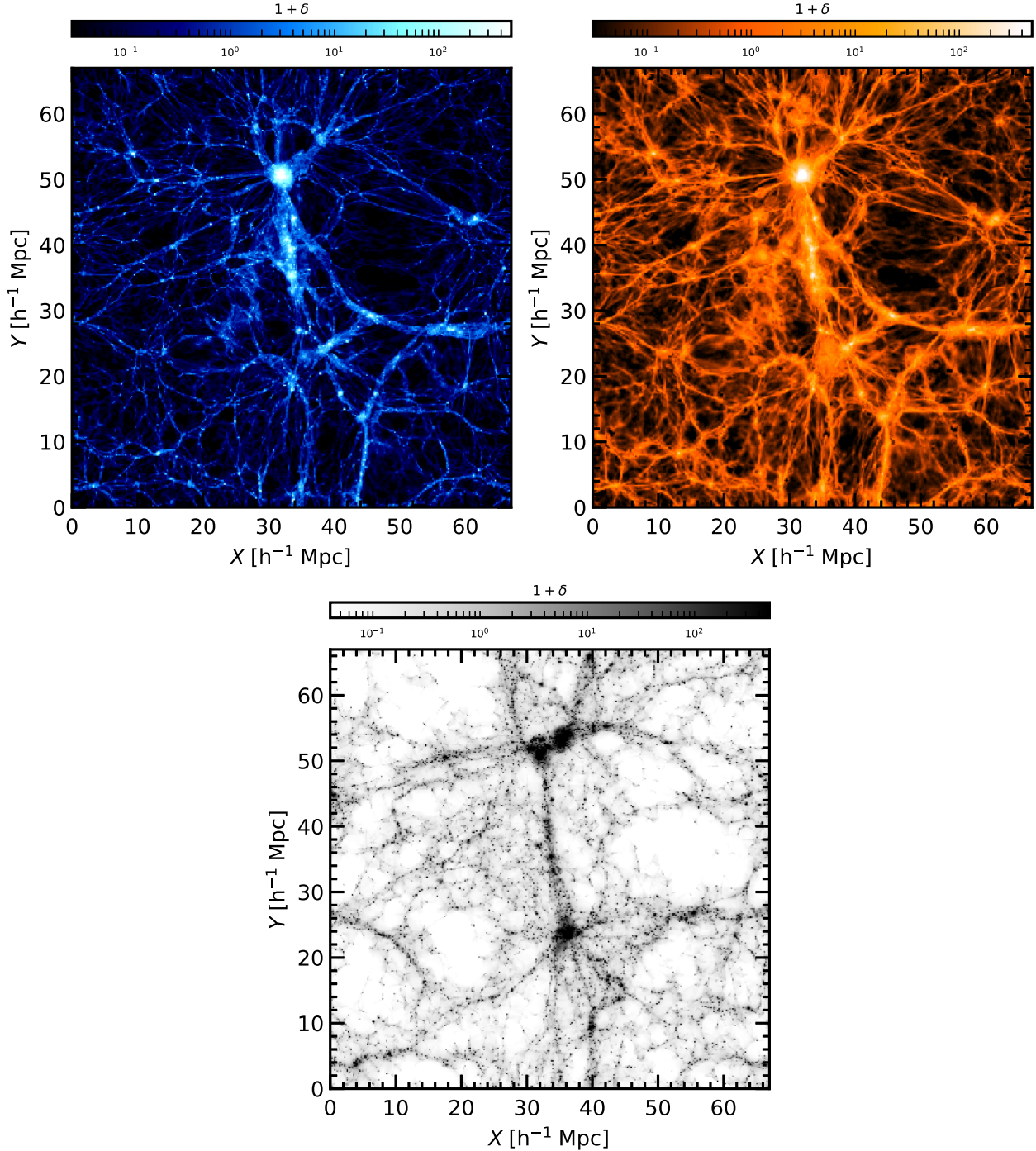
Figure 1. Dark matter, gas, and stellar density fields: Dark matter (top left) and gas (top right) density distributions in a thin slice ( 132 h^{-1} \text{ kpc} ) of the EAGLE simulation. Lower panel: stellar density field in a thick slice ( 10 h^{-1} \text{ Mpc} ) centred on the thin slice shown in the top panels. The logarithmically scaled colour bar represents the density contrast, 1 + \delta .
