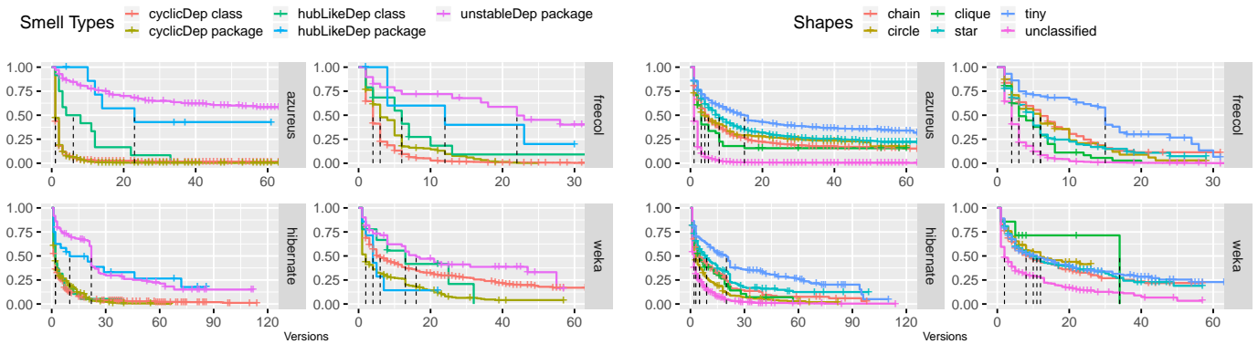
(a) Smells of different types affecting classes or packages.
